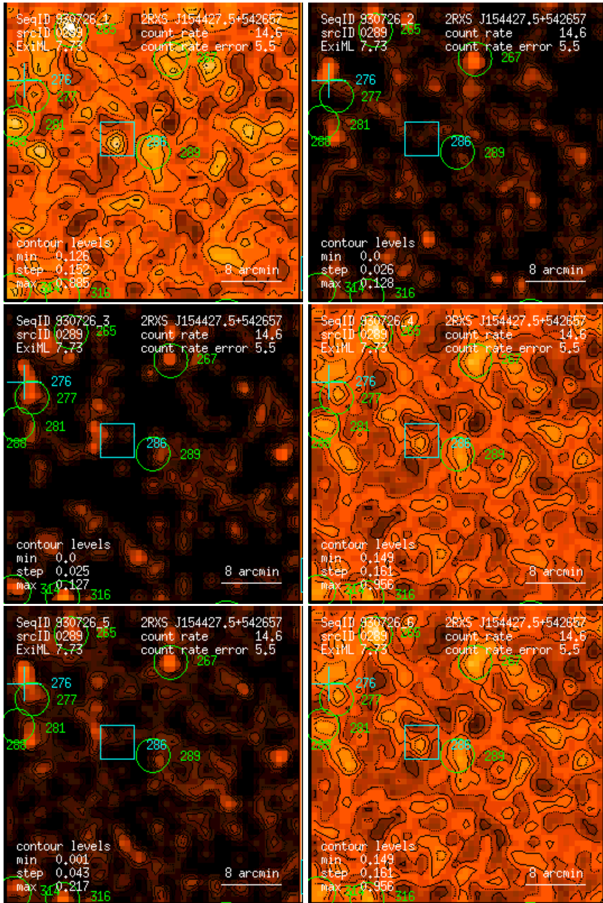
Figure 289: RASS 930726: detection 0289: band rate images, Gaussian filter: (1) PSPC channels 11 – 41, (2) 52 – 90, (3) 91 – 201, (4) 11 – 235, (5) 52 – 201, (6) 11 – 201. Broad band rates in counts/ks. Band rate contour levels in counts/ks/arcmin 2 .
