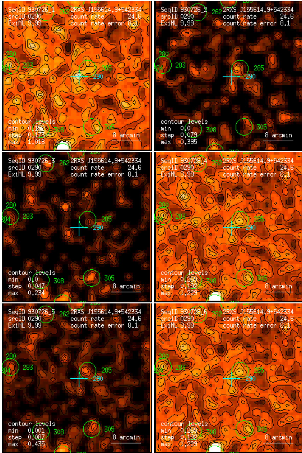
Figure 290: RASS 930726: detection 0290: band rate images, Gaussian filter: (1) PSPC channels 11 – 41, (2) 52 – 90, (3) 91 – 201, (4) 11 – 235, (5) 52 – 201, (6) 11 – 201. Broad band rates in counts/ks. Band rate contour levels in counts/ks/arcmin 2 .
