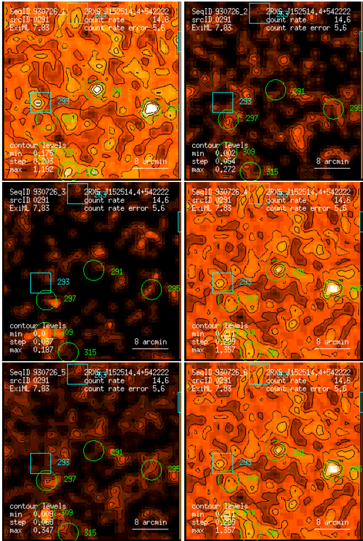
Figure 291: RASS 930726: detection 0291: band rate images, Gaussian filter: (1) PSPC channels 11 – 41, (2) 52 – 90, (3) 91 – 201, (4) 11 – 235, (5) 52 – 201, (6) 11 – 201. Broad band rates in counts/ks. Band rate contour levels in counts/ks/arcmin 2 .
