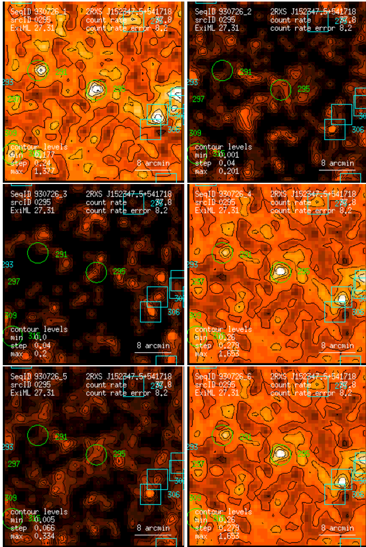
Figure 295: RASS 930726: detection 0295: band rate images, Gaussian filter: (1) PSPC channels 11 – 41, (2) 52 – 90, (3) 91 – 201, (4) 11 – 235, (5) 52 – 201, (6) 11 – 201. Broad band rates in counts/ks. Band rate contour levels in counts/ks/arcmin 2 .
