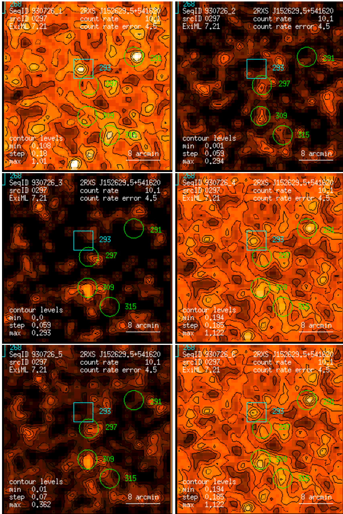
Figure 297: RASS 930726: detection 0297: band rate images, Gaussian filter: (1) PSPC channels 11 – 41, (2) 52 – 90, (3) 91 – 201, (4) 11 – 235, (5) 52 – 201, (6) 11 – 201. Broad band rates in counts/ks. Band rate contour levels in counts/ks/arcmin 2 .
