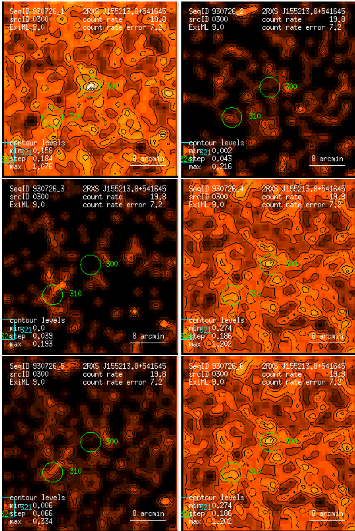
Figure 300: RASS 930726: detection 0300: band rate images, Gaussian filter: (1) PSPC channels 11 – 41, (2) 52 – 90, (3) 91 – 201, (4) 11 – 235, (5) 52 – 201, (6) 11 – 201. Broad band rates in counts/ks. Band rate contour levels in counts/ks/arcmin 2 .
