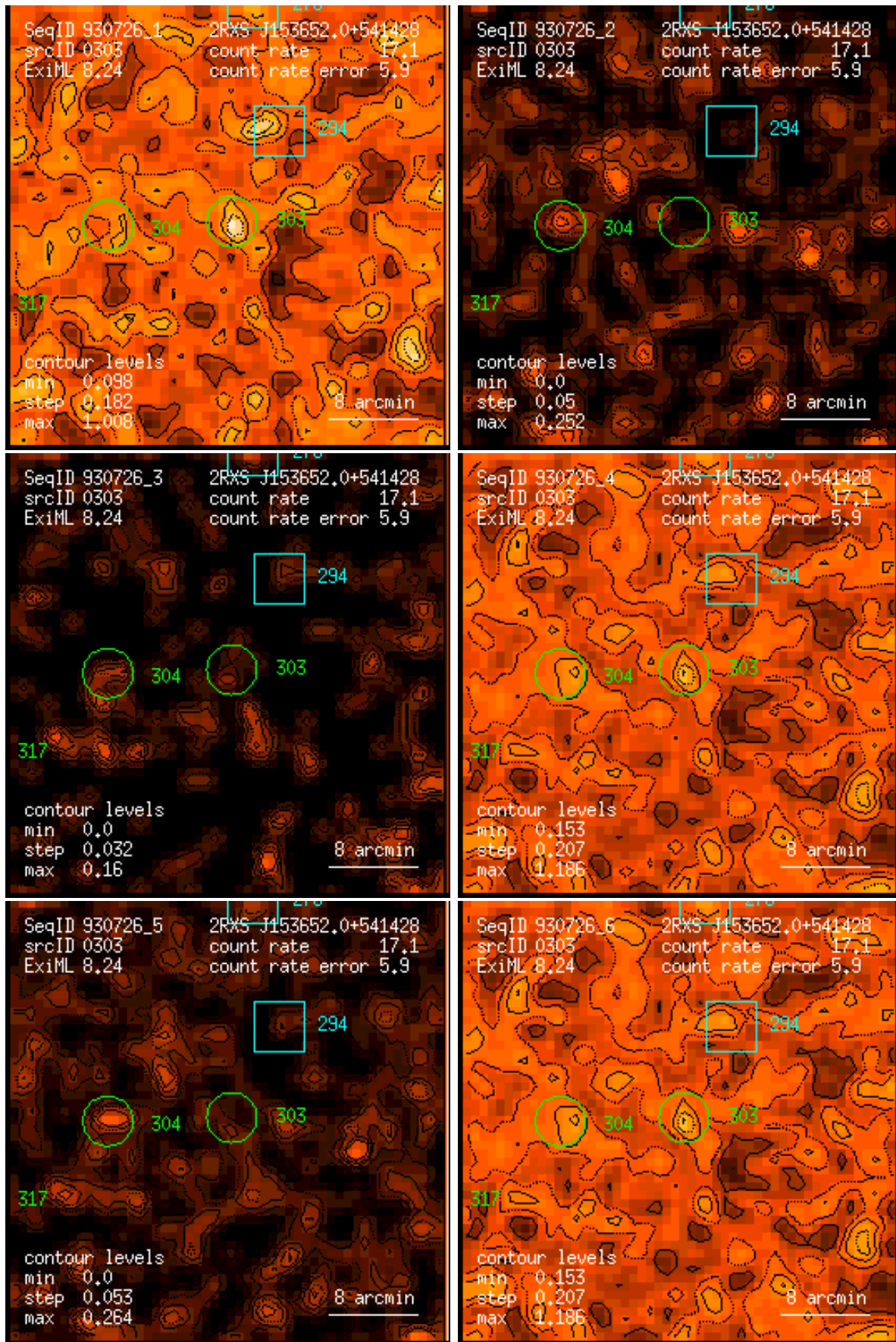
Figure 303: RASS 930726: detection 0303: band rate images, Gaussian filter: (1) PSPC channels 11 – 41, (2) 52 – 90, (3) 91 – 201, (4) 11 – 235, (5) 52 – 201, (6) 11 – 201. Broad band rates in counts/ks. Band rate contour levels in counts/ks/arcmin 2 .
