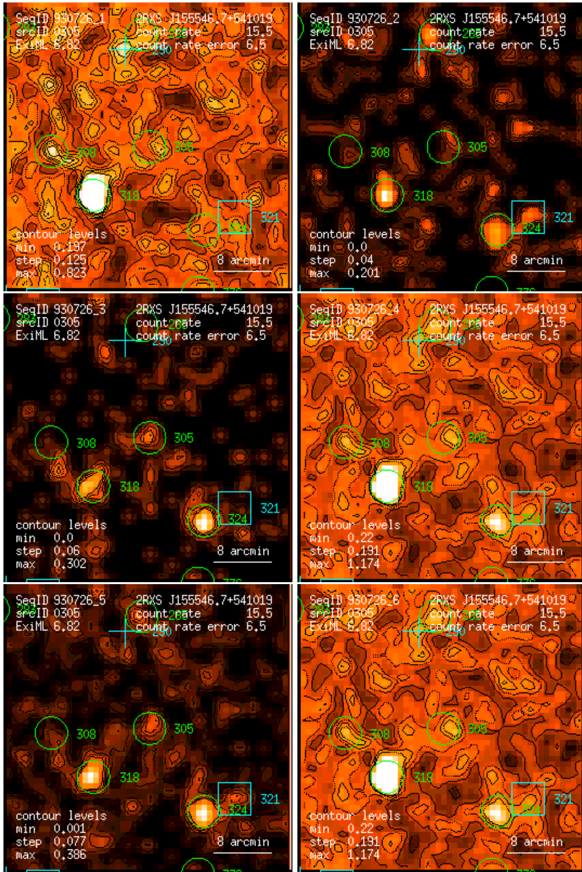
Figure 305: RASS 930726: detection 0305: band rate images, Gaussian filter: (1) PSPC channels 11 – 41, (2) 52 – 90, (3) 91 – 201, (4) 11 – 235, (5) 52 – 201, (6) 11 – 201. Broad band rates in counts/ks. Band rate contour levels in counts/ks/arcmin 2 .
