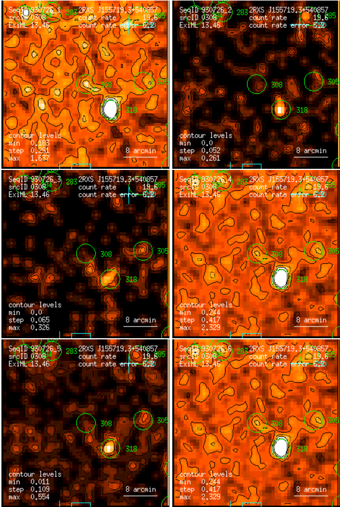
Figure 308: RASS 930726: detection 0308: band rate images, Gaussian filter: (1) PSPC channels 11 – 41, (2) 52 – 90, (3) 91 – 201, (4) 11 – 235, (5) 52 – 201, (6) 11 – 201. Broad band rates in counts/ks. Band rate contour levels in counts/ks/arcmin 2 .
