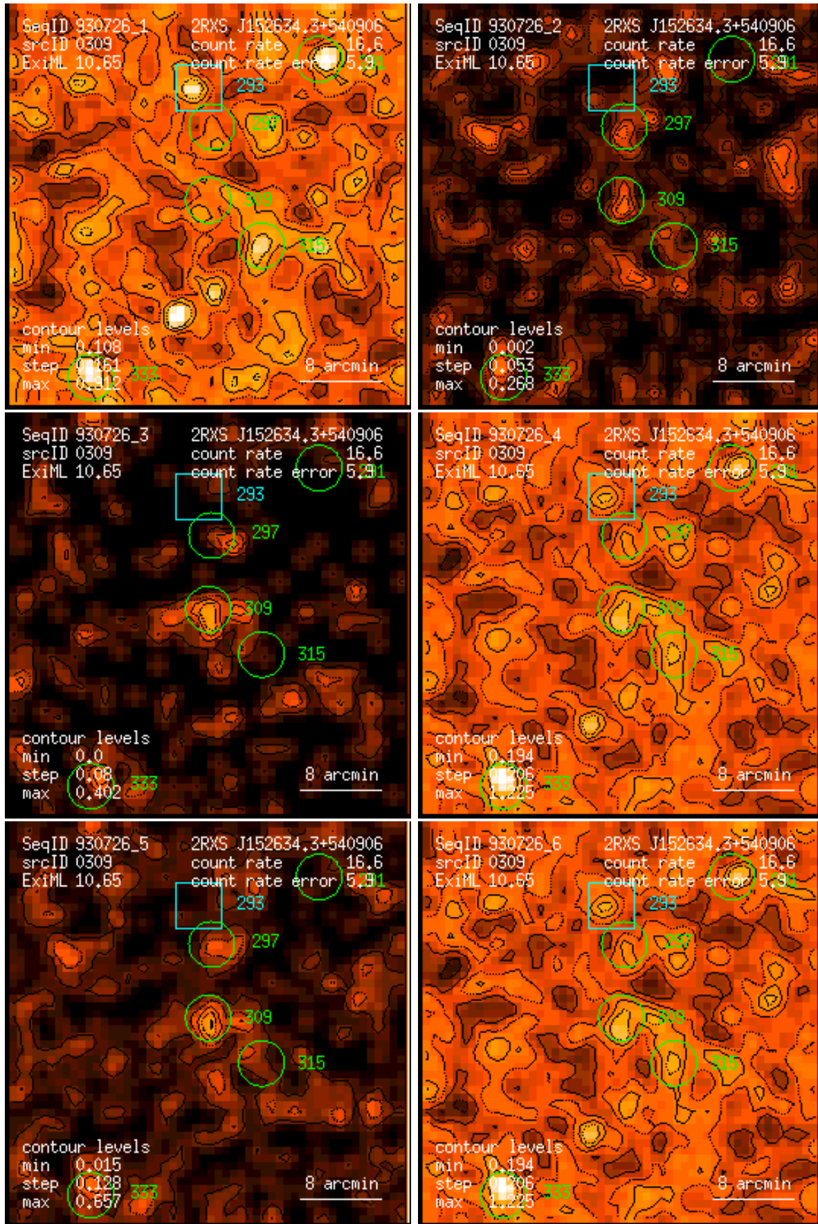
Figure 309: RASS 930726: detection 0309: band rate images, Gaussian filter: (1) PSPC channels 11 – 41, (2) 52 – 90, (3) 91 – 201, (4) 11 – 235, (5) 52 – 201, (6) 11 – 201. Broad band rates in counts/ks. Band rate contour levels in counts/ks/arcmin 2 .
