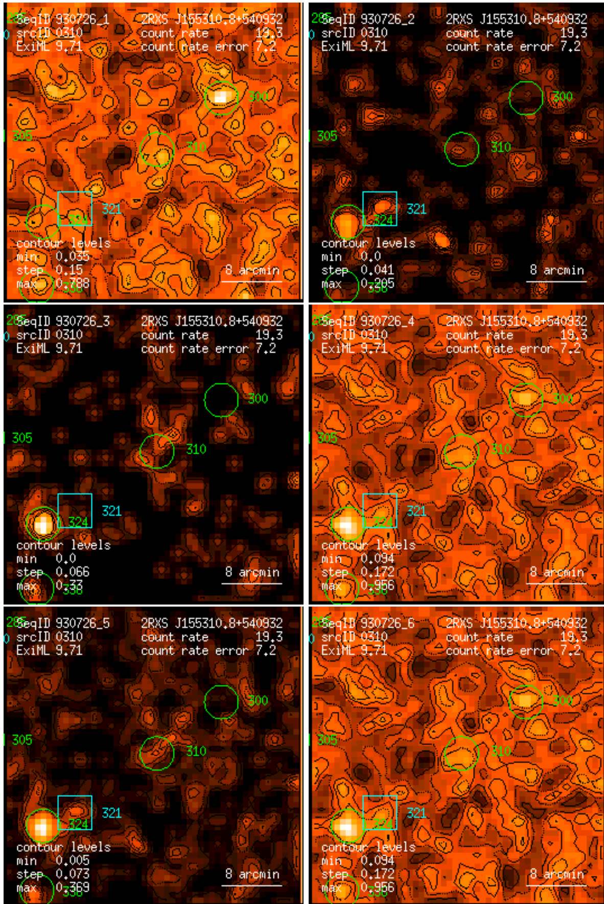
Figure 310: RASS 930726: detection 0310: band rate images, Gaussian filter: (1) PSPC channels 11 – 41, (2) 52 – 90, (3) 91 – 201, (4) 11 – 235, (5) 52 – 201, (6) 11 – 201. Broad band rates in counts/ks. Band rate contour levels in counts/ks/arcmin 2 .
