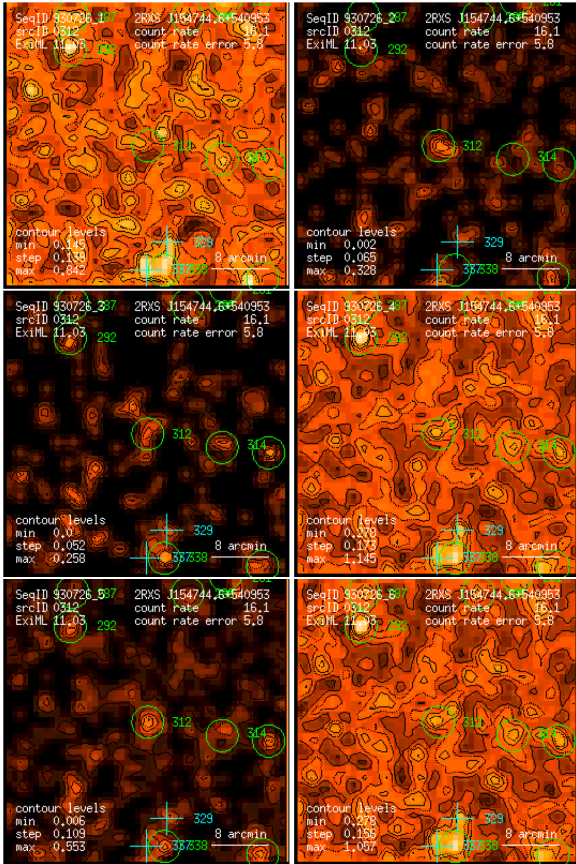
Figure 312: RASS 930726: detection 0312: band rate images, Gaussian filter: (1) PSPC channels 11 – 41, (2) 52 – 90, (3) 91 – 201, (4) 11 – 235, (5) 52 – 201, (6) 11 – 201. Broad band rates in counts/ks. Band rate contour levels in counts/ks/arcmin 2 .
