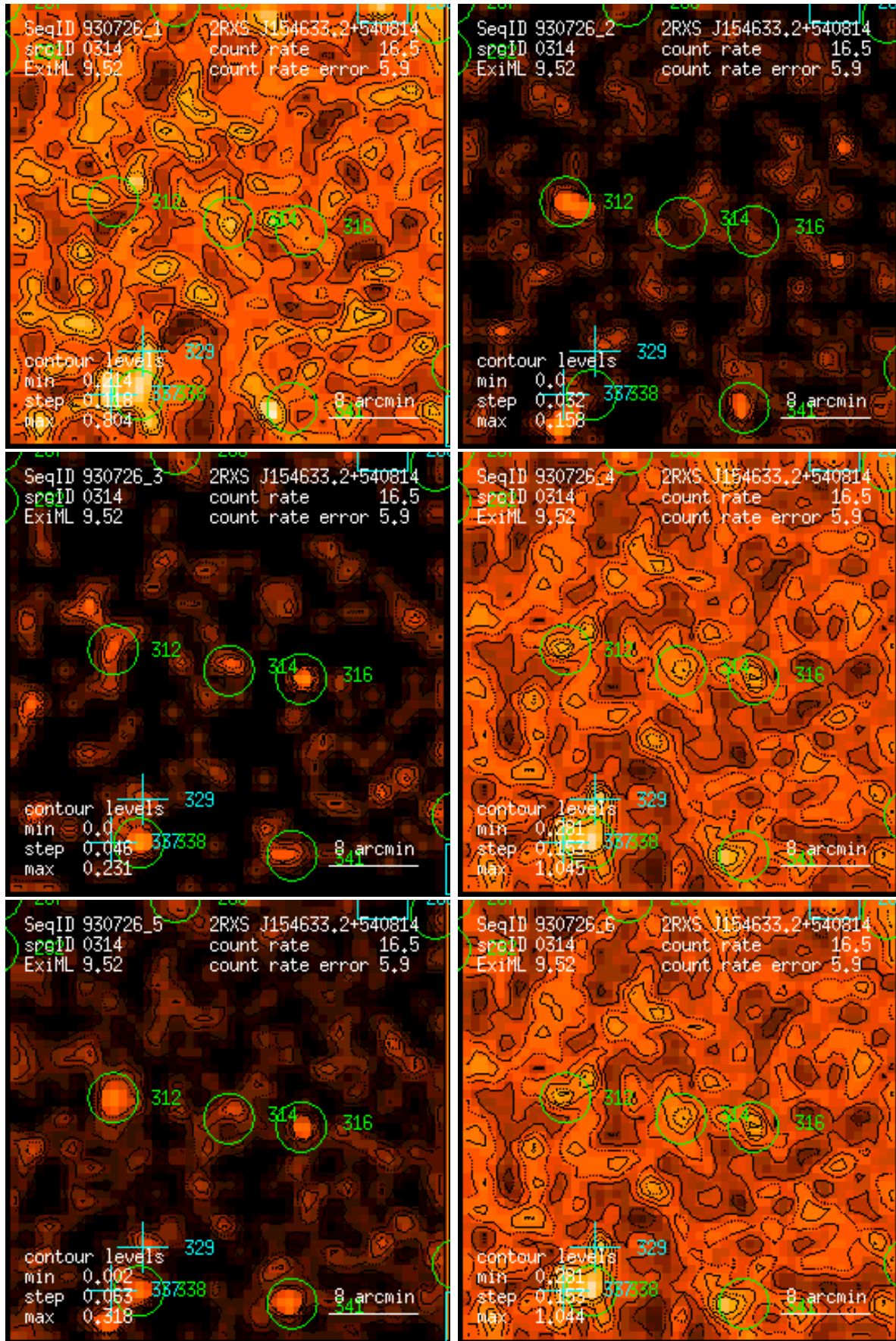
Figure 314: RASS 930726: detection 0314: band rate images, Gaussian filter: (1) PSPC channels 11 – 41, (2) 52 – 90, (3) 91 – 201, (4) 11 – 235, (5) 52 – 201, (6) 11 – 201. Broad band rates in counts/ks. Band rate contour levels in counts/ks/arcmin 2 .
