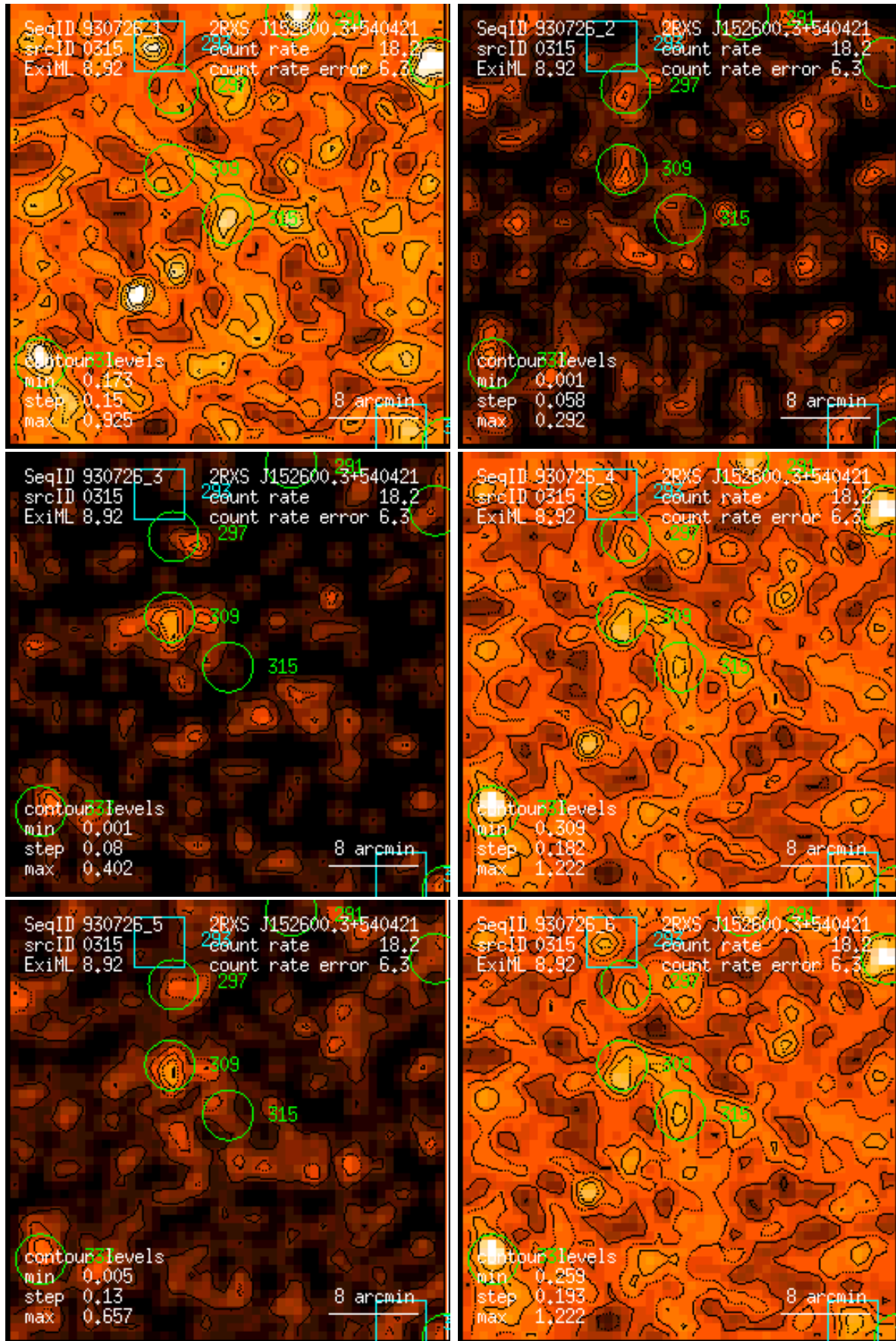
Figure 315: RASS 930726: detection 0315: band rate images, Gaussian filter: (1) PSPC channels 11 – 41, (2) 52 – 90, (3) 91 – 201, (4) 11 – 235, (5) 52 – 201, (6) 11 – 201. Broad band rates in counts/ks. Band rate contour levels in counts/ks/arcmin 2 .
