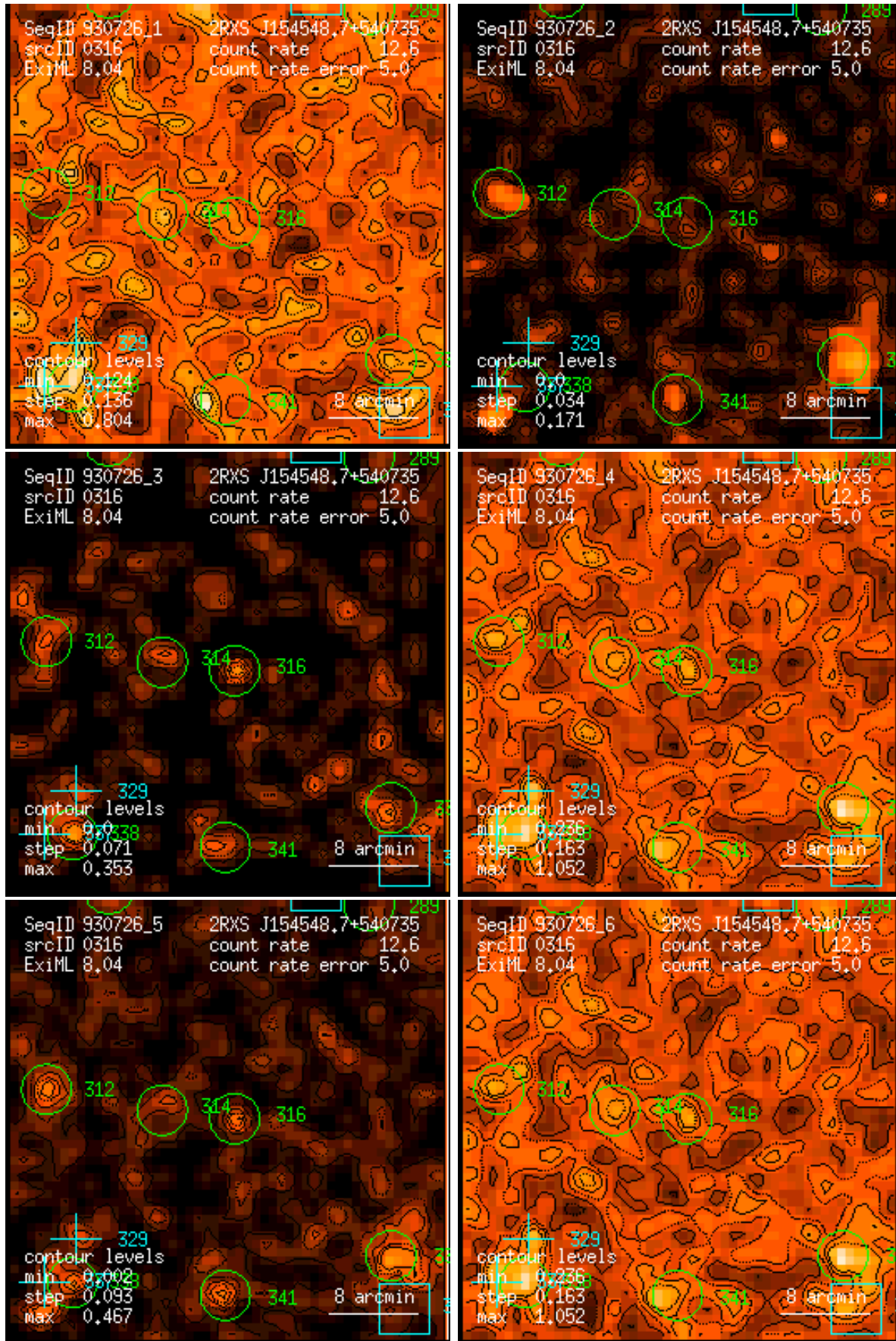
Figure 316: RASS 930726: detection 0316: band rate images, Gaussian filter: (1) PSPC channels 11 – 41, (2) 52 – 90, (3) 91 – 201, (4) 11 – 235, (5) 52 – 201, (6) 11 – 201. Broad band rates in counts/ks. Band rate contour levels in counts/ks/arcmin 2 .
