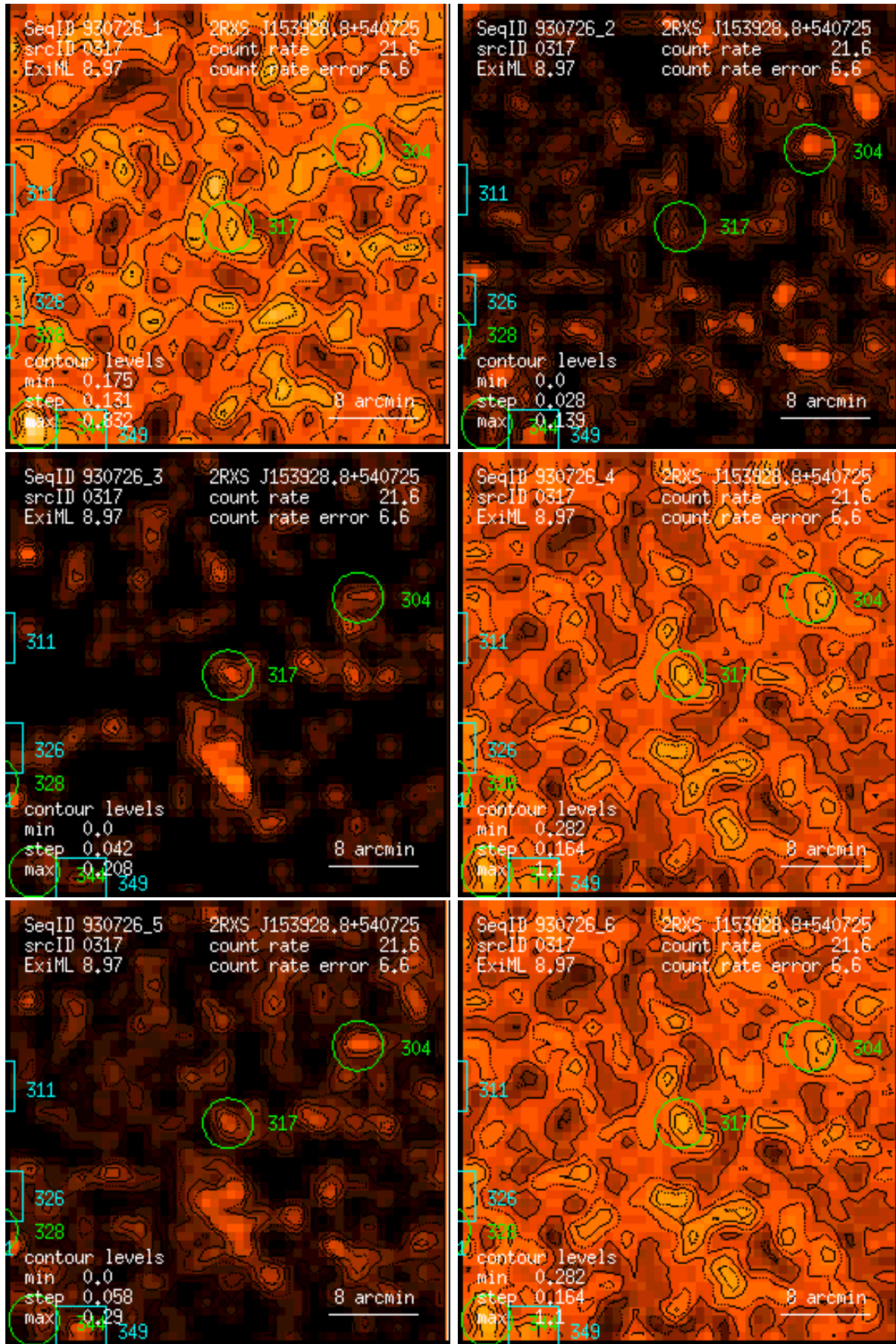
Figure 317: RASS 930726: detection 0317: band rate images, Gaussian filter: (1) PSPC channels 11 – 41, (2) 52 – 90, (3) 91 – 201, (4) 11 – 235, (5) 52 – 201, (6) 11 – 201. Broad band rates in counts/ks. Band rate contour levels in counts/ks/arcmin 2 .
