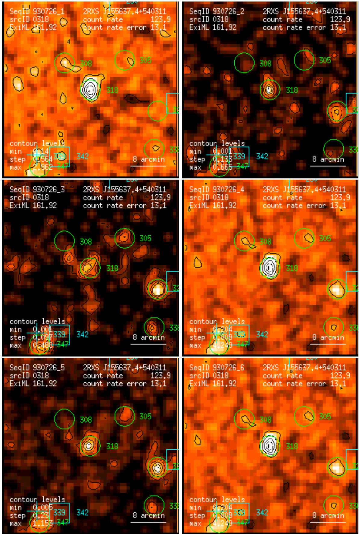
Figure 318: RASS 930726: detection 0318: band rate images, Gaussian filter: (1) PSPC channels 11 – 41, (2) 52 – 90, (3) 91 – 201, (4) 11 – 235, (5) 52 – 201, (6) 11 – 201. Broad band rates in counts/ks. Band rate contour levels in counts/ks/arcmin 2 .
