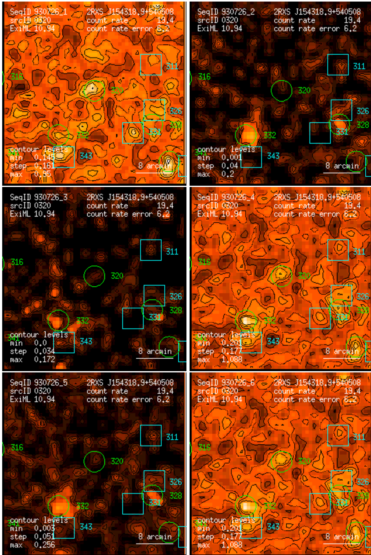
Figure 320: RASS 930726: detection 0320: band rate images, Gaussian filter: (1) PSPC channels 11 – 41, (2) 52 – 90, (3) 91 – 201, (4) 11 – 235, (5) 52 – 201, (6) 11 – 201. Broad band rates in counts/ks. Band rate contour levels in counts/ks/arcmin 2 .
