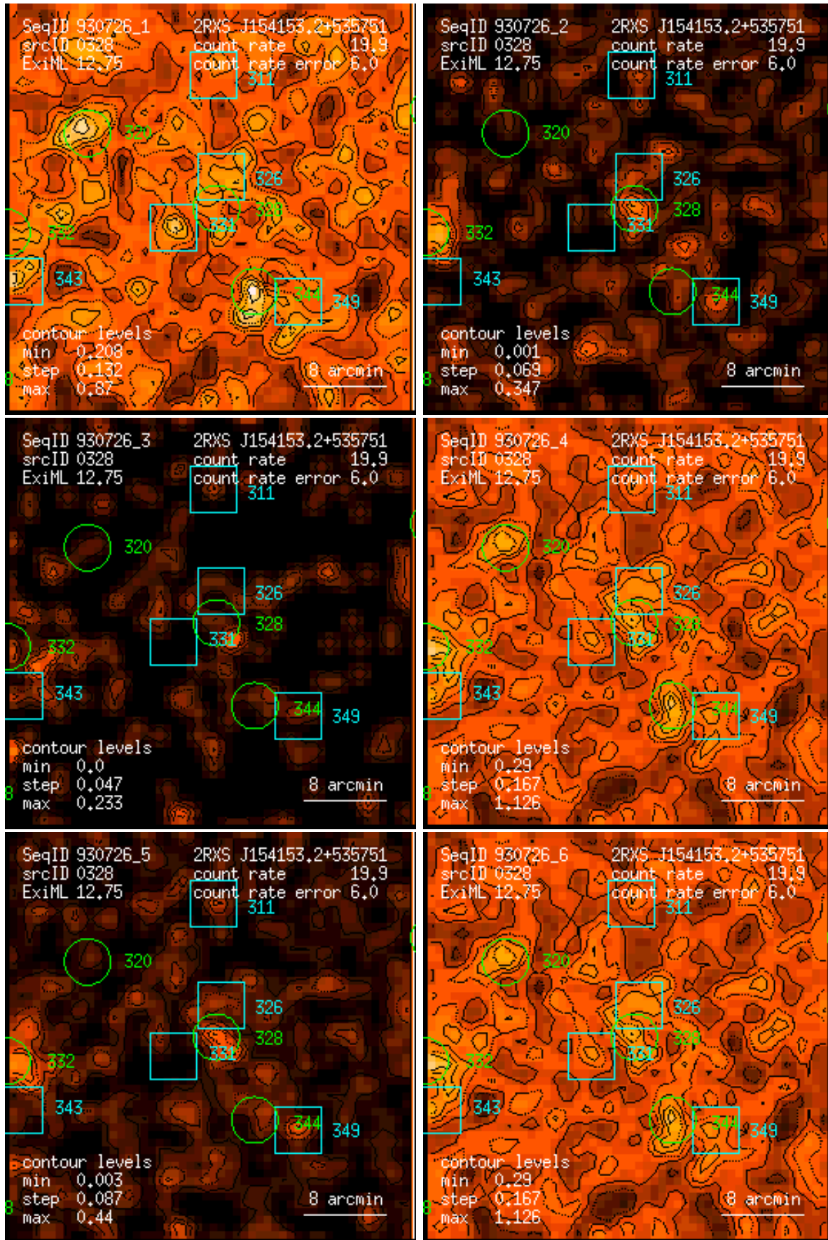
Figure 328: RASS 930726: detection 0328: band rate images, Gaussian filter: (1) PSPC channels 11 – 41, (2) 52 – 90, (3) 91 – 201, (4) 11 – 235, (5) 52 – 201, (6) 11 – 201. Broad band rates in counts/ks. Band rate contour levels in counts/ks/arcmin 2 .
