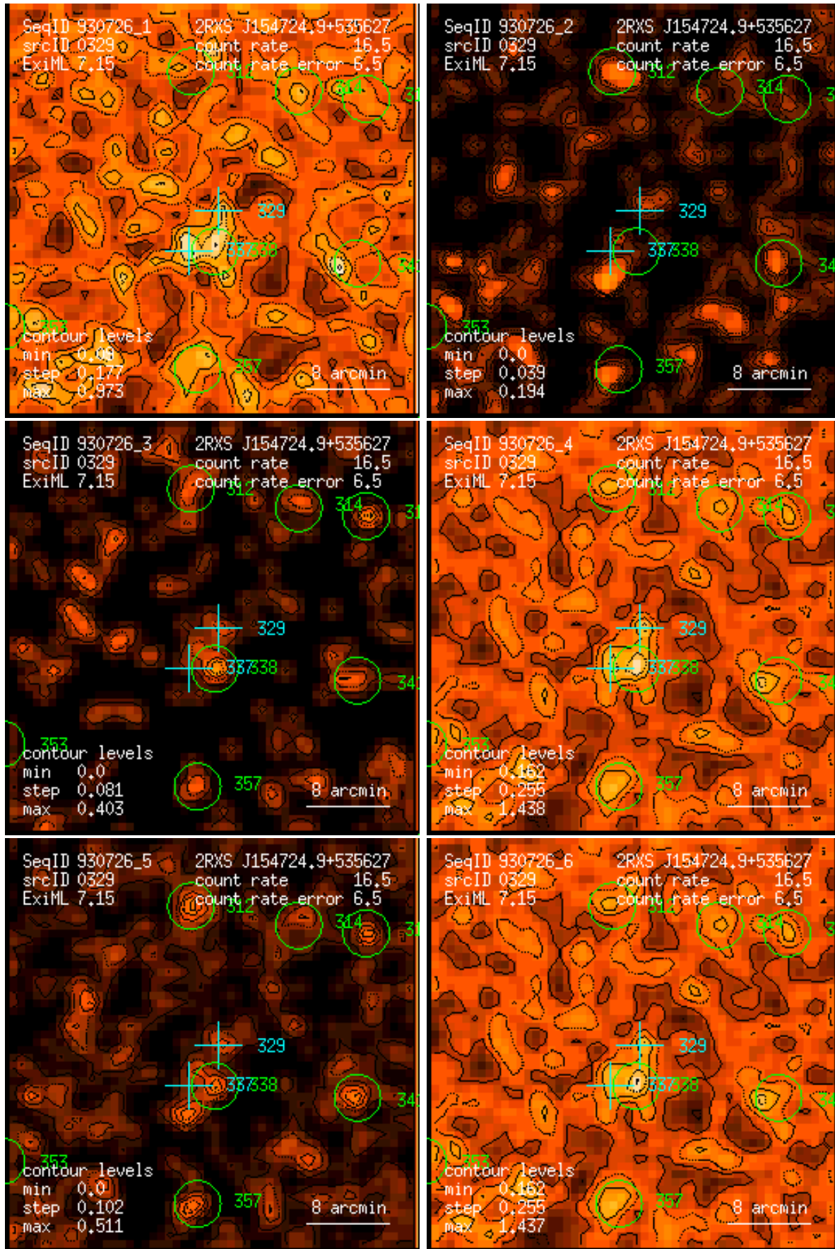
Figure 329: RASS 930726: detection 0329: band rate images, Gaussian filter: (1) PSPC channels 11 – 41, (2) 52 – 90, (3) 91 – 201, (4) 11 – 235, (5) 52 – 201, (6) 11 – 201. Broad band rates in counts/ks. Band rate contour levels in counts/ks/arcmin 2 .
