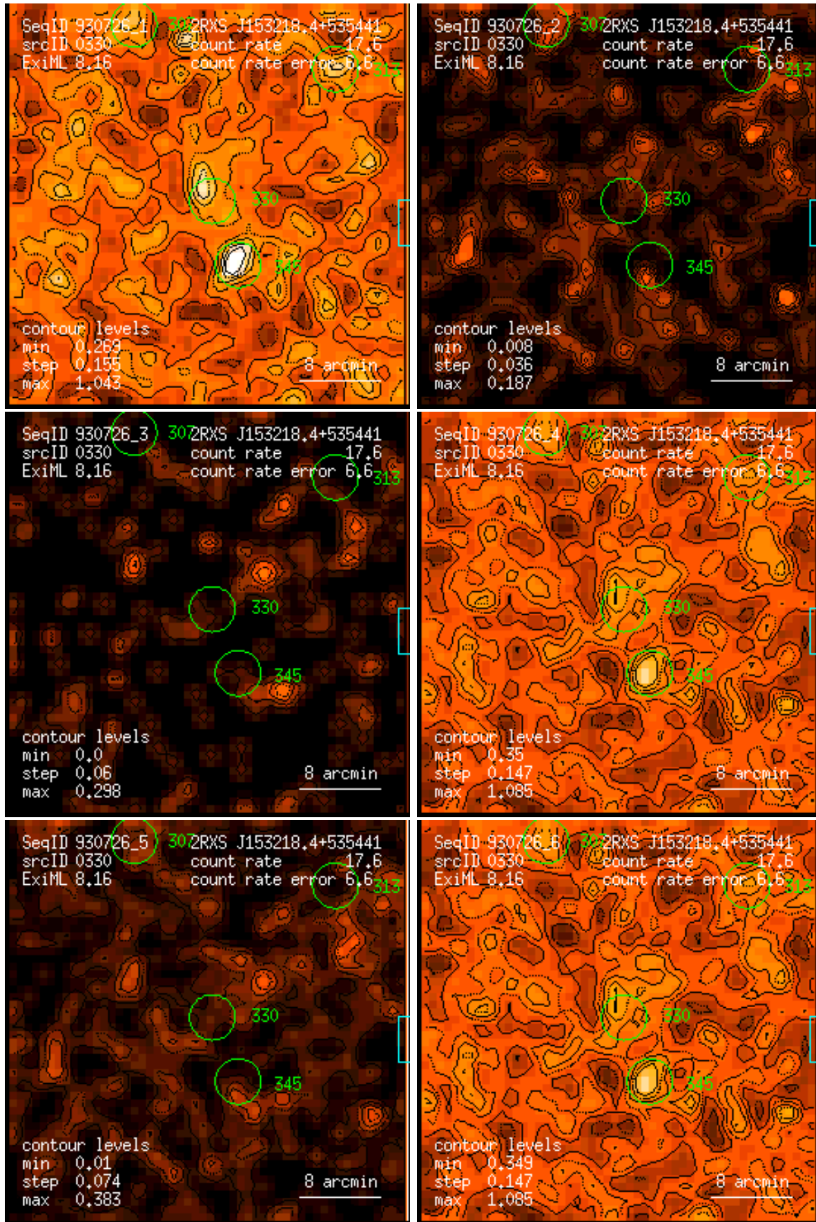
Figure 330: RASS 930726: detection 0330: band rate images, Gaussian filter: (1) PSPC channels 11 – 41, (2) 52 – 90, (3) 91 – 201, (4) 11 – 235, (5) 52 – 201, (6) 11 – 201. Broad band rates in counts/ks. Band rate contour levels in counts/ks/arcmin 2 .
