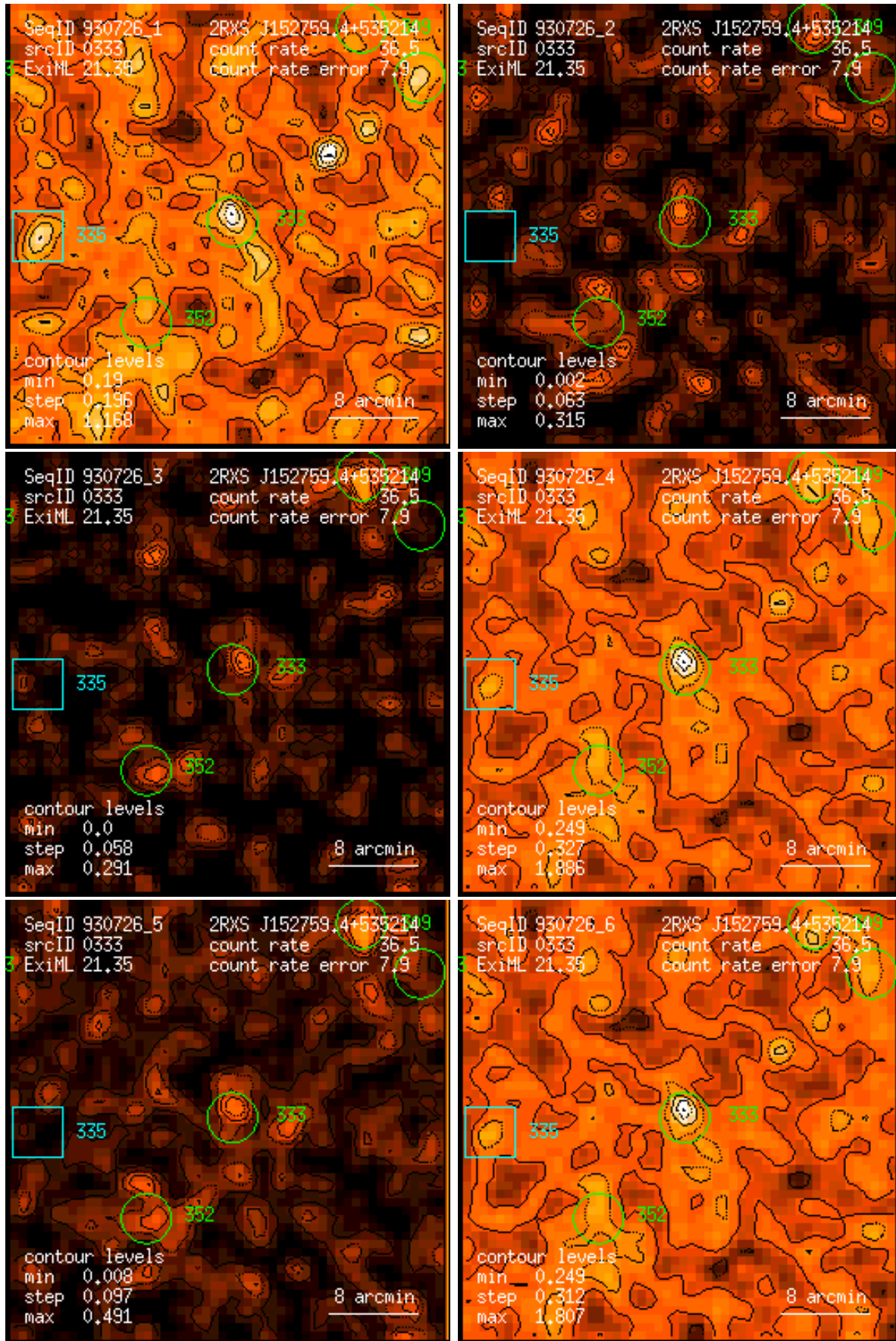
Figure 333: RASS 930726: detection 0333: band rate images, Gaussian filter: (1) PSPC channels 11 – 41, (2) 52 – 90, (3) 91 – 201, (4) 11 – 235, (5) 52 – 201, (6) 11 – 201. Broad band rates in counts/ks. Band rate contour levels in counts/ks/arcmin 2 .
