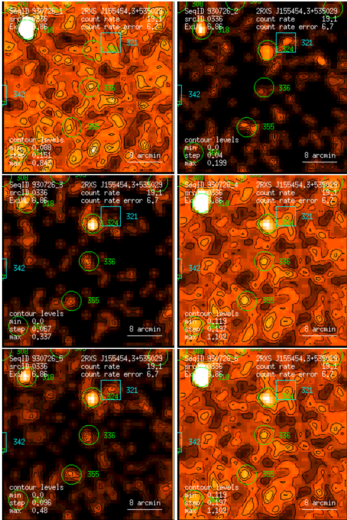
Figure 336: RASS 930726: detection 0336: band rate images, Gaussian filter: (1) PSPC channels 11 – 41, (2) 52 – 90, (3) 91 – 201, (4) 11 – 235, (5) 52 – 201, (6) 11 – 201. Broad band rates in counts/ks. Band rate contour levels in counts/ks/arcmin 2 .
