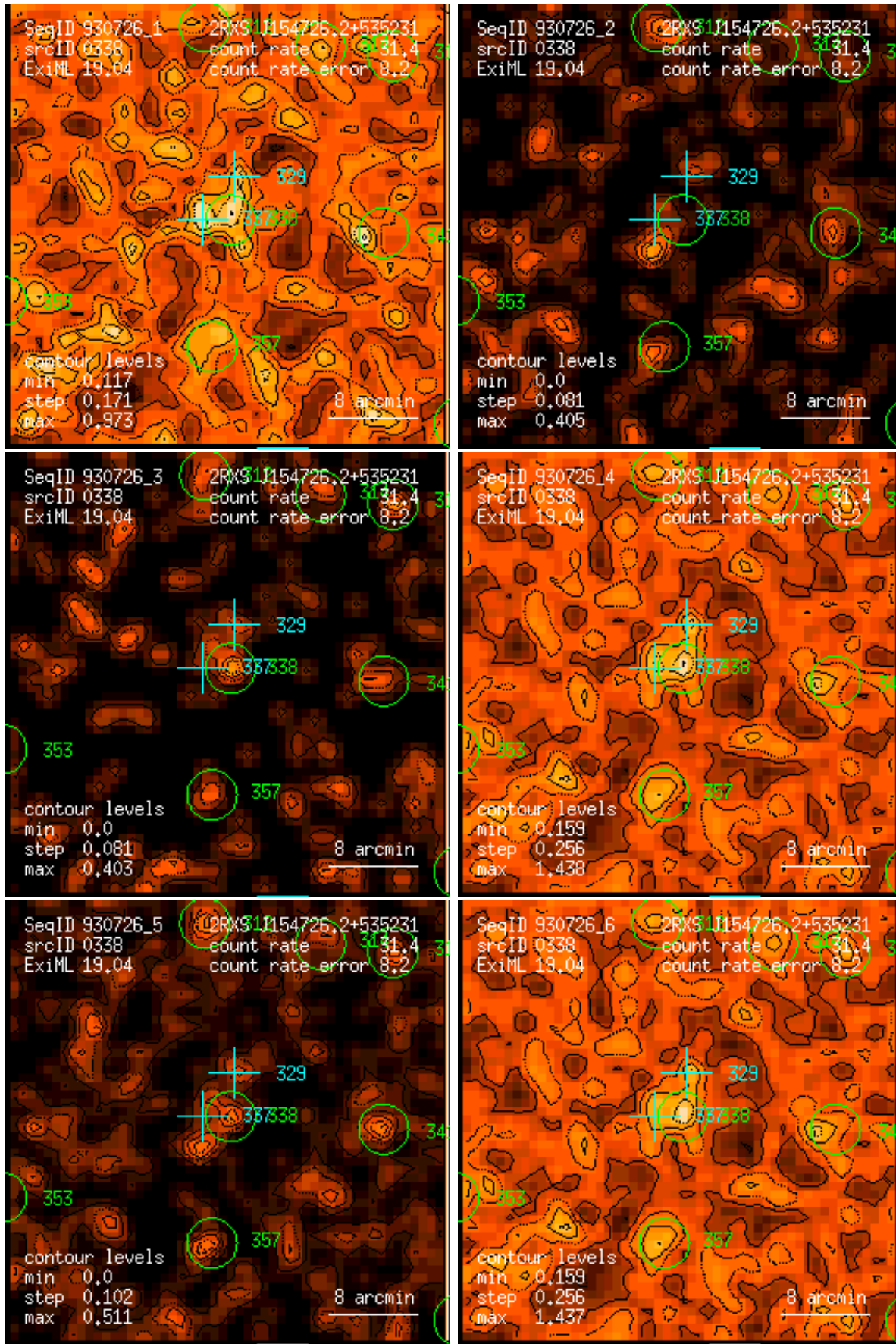
Figure 338: RASS 930726: detection 0338: band rate images, Gaussian filter: (1) PSPC channels 11 – 41, (2) 52 – 90, (3) 91 – 201, (4) 11 – 235, (5) 52 – 201, (6) 11 – 201. Broad band rates in counts/ks. Band rate contour levels in counts/ks/arcmin 2 .
