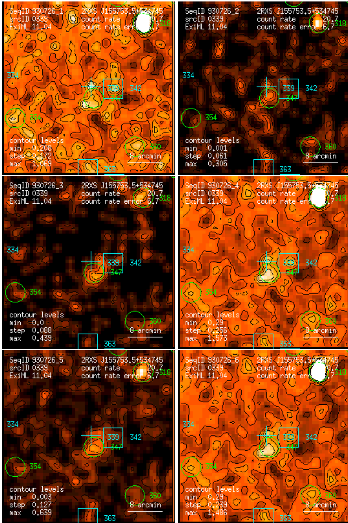
Figure 339: RASS 930726: detection 0339: band rate images, Gaussian filter: (1) PSPC channels 11 – 41, (2) 52 – 90, (3) 91 – 201, (4) 11 – 235, (5) 52 – 201, (6) 11 – 201. Broad band rates in counts/ks. Band rate contour levels in counts/ks/arcmin 2 .
