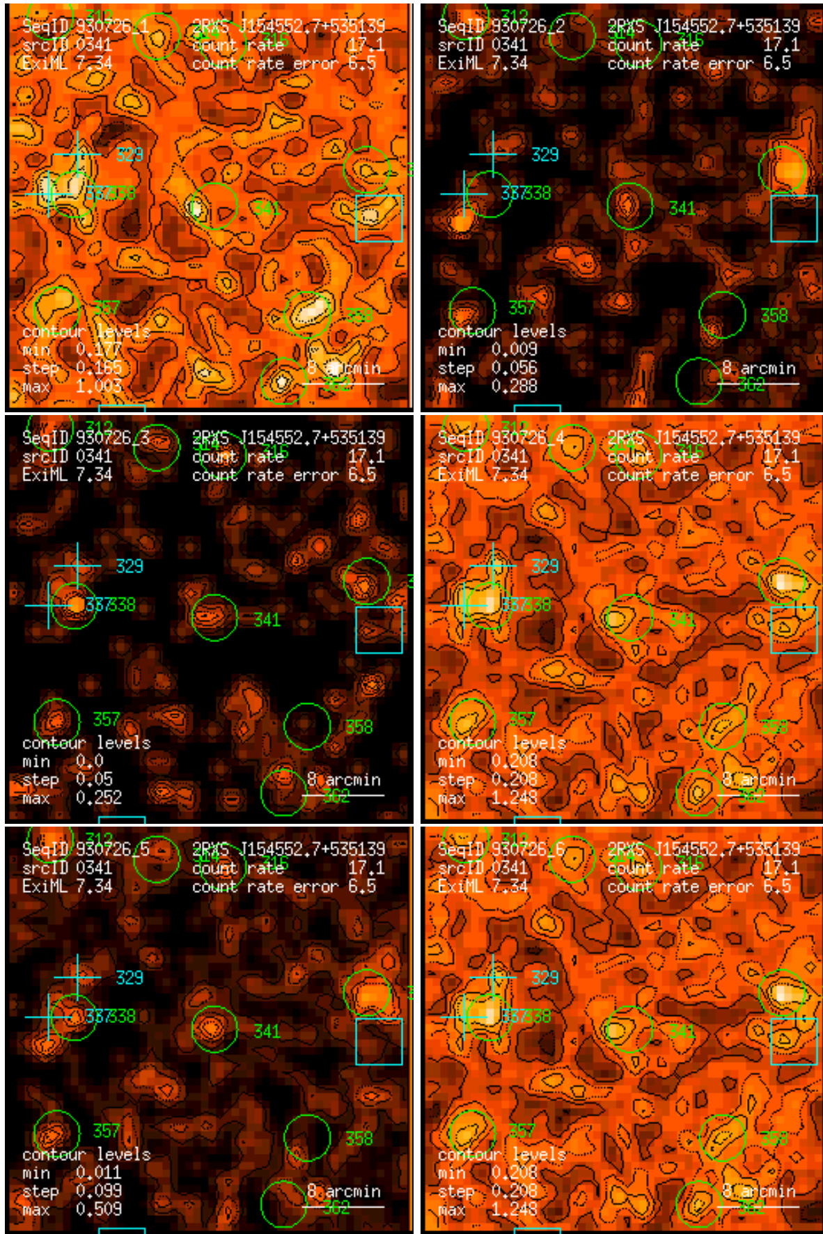
Figure 341: RASS 930726: detection 0341: band rate images, Gaussian filter: (1) PSPC channels 11 – 41, (2) 52 – 90, (3) 91 – 201, (4) 11 – 235, (5) 52 – 201, (6) 11 – 201. Broad band rates in counts/ks. Band rate contour levels in counts/ks/arcmin 2 .
