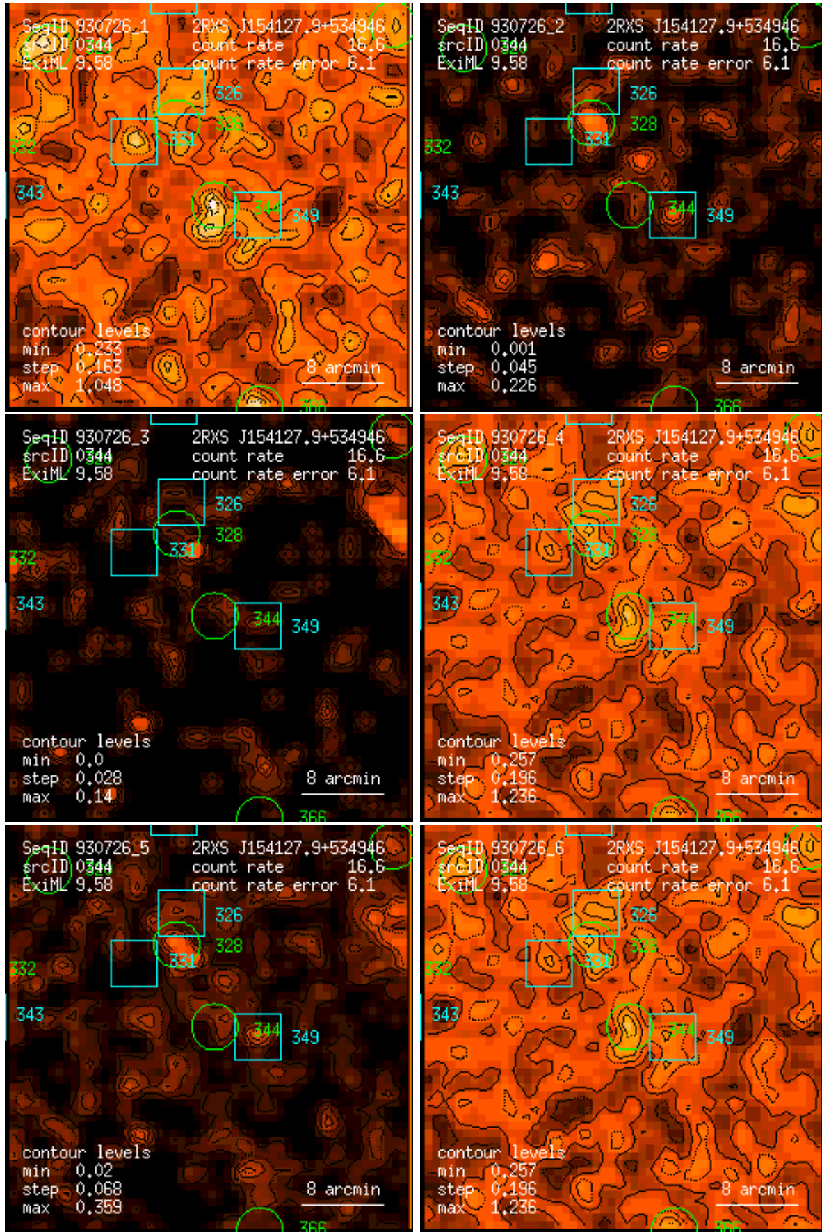
Figure 344: RASS 930726: detection 0344: band rate images, Gaussian filter: (1) PSPC channels 11 – 41, (2) 52 – 90, (3) 91 – 201, (4) 11 – 235, (5) 52 – 201, (6) 11 – 201. Broad band rates in counts/ks. Band rate contour levels in counts/ks/arcmin 2 .
