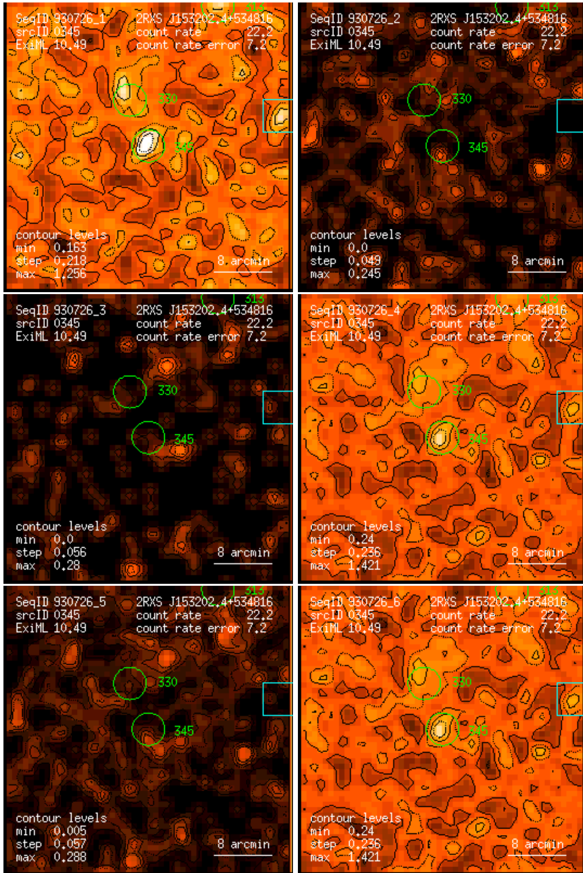
Figure 345: RASS 930726: detection 0345: band rate images, Gaussian filter: (1) PSPC channels 11 – 41, (2) 52 – 90, (3) 91 – 201, (4) 11 – 235, (5) 52 – 201, (6) 11 – 201. Broad band rates in counts/ks. Band rate contour levels in counts/ks/arcmin 2 .
