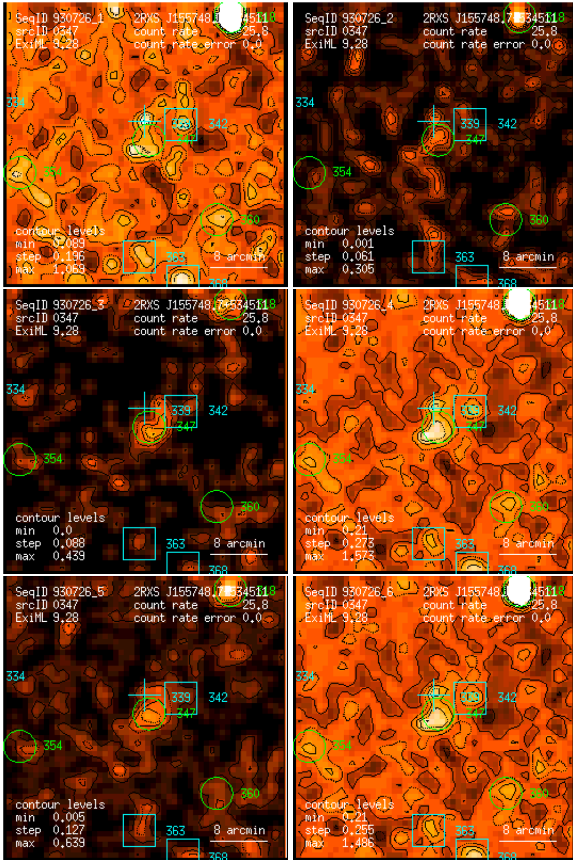
Figure 347: RASS 930726: detection 0347: band rate images, Gaussian filter: (1) PSPC channels 11 – 41, (2) 52 – 90, (3) 91 – 201, (4) 11 – 235, (5) 52 – 201, (6) 11 – 201. Broad band rates in counts/ks. Band rate contour levels in counts/ks/arcmin 2 .
