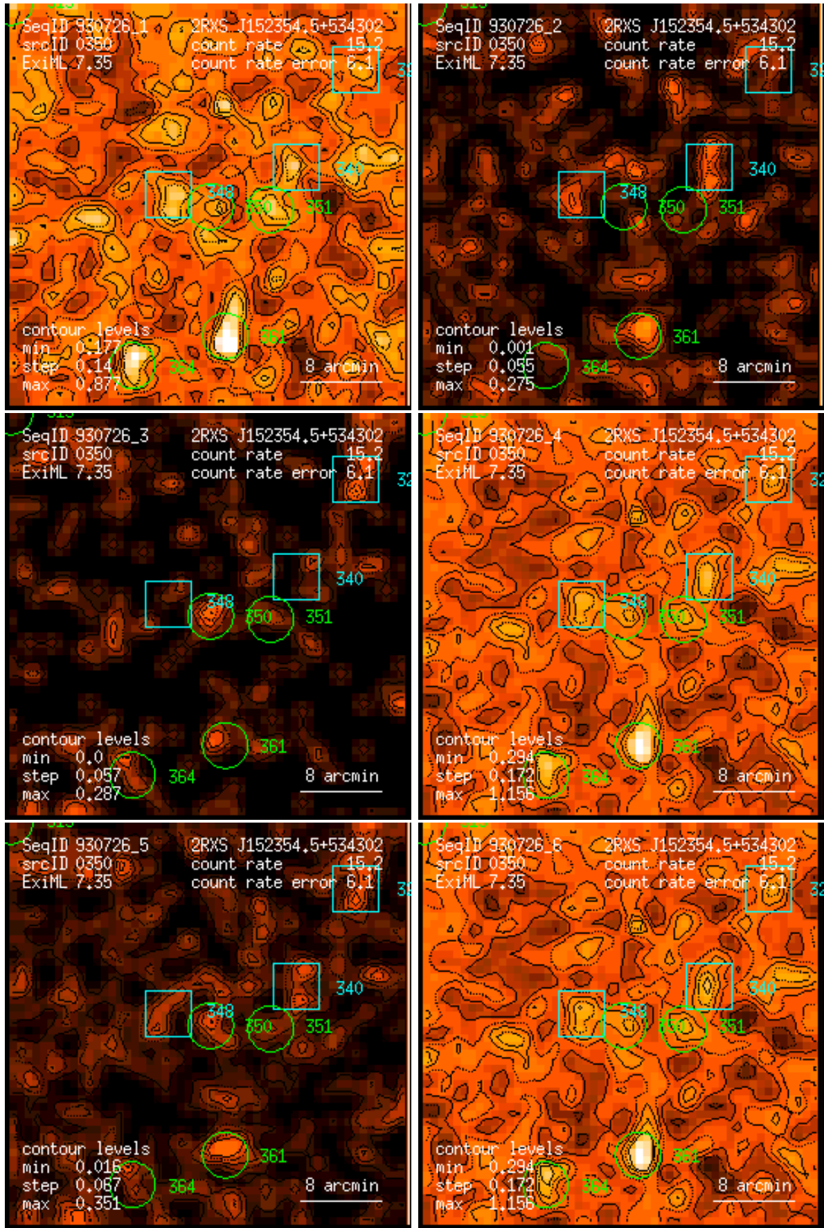
Figure 350: RASS 930726: detection 0350: band rate images, Gaussian filter: (1) PSPC channels 11 – 41, (2) 52 – 90, (3) 91 – 201, (4) 11 – 235, (5) 52 – 201, (6) 11 – 201. Broad band rates in counts/ks. Band rate contour levels in counts/ks/arcmin 2 .
