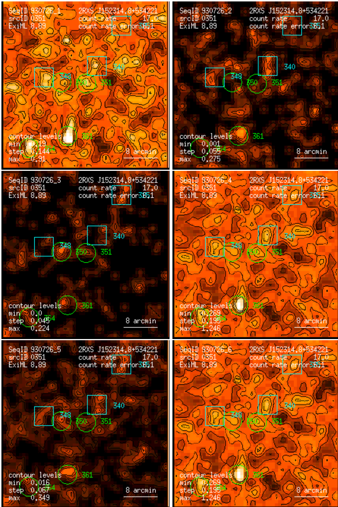
Figure 351: RASS 930726: detection 0351: band rate images, Gaussian filter: (1) PSPC channels 11 – 41, (2) 52 – 90, (3) 91 – 201, (4) 11 – 235, (5) 52 – 201, (6) 11 – 201. Broad band rates in counts/ks. Band rate contour levels in counts/ks/arcmin 2 .
