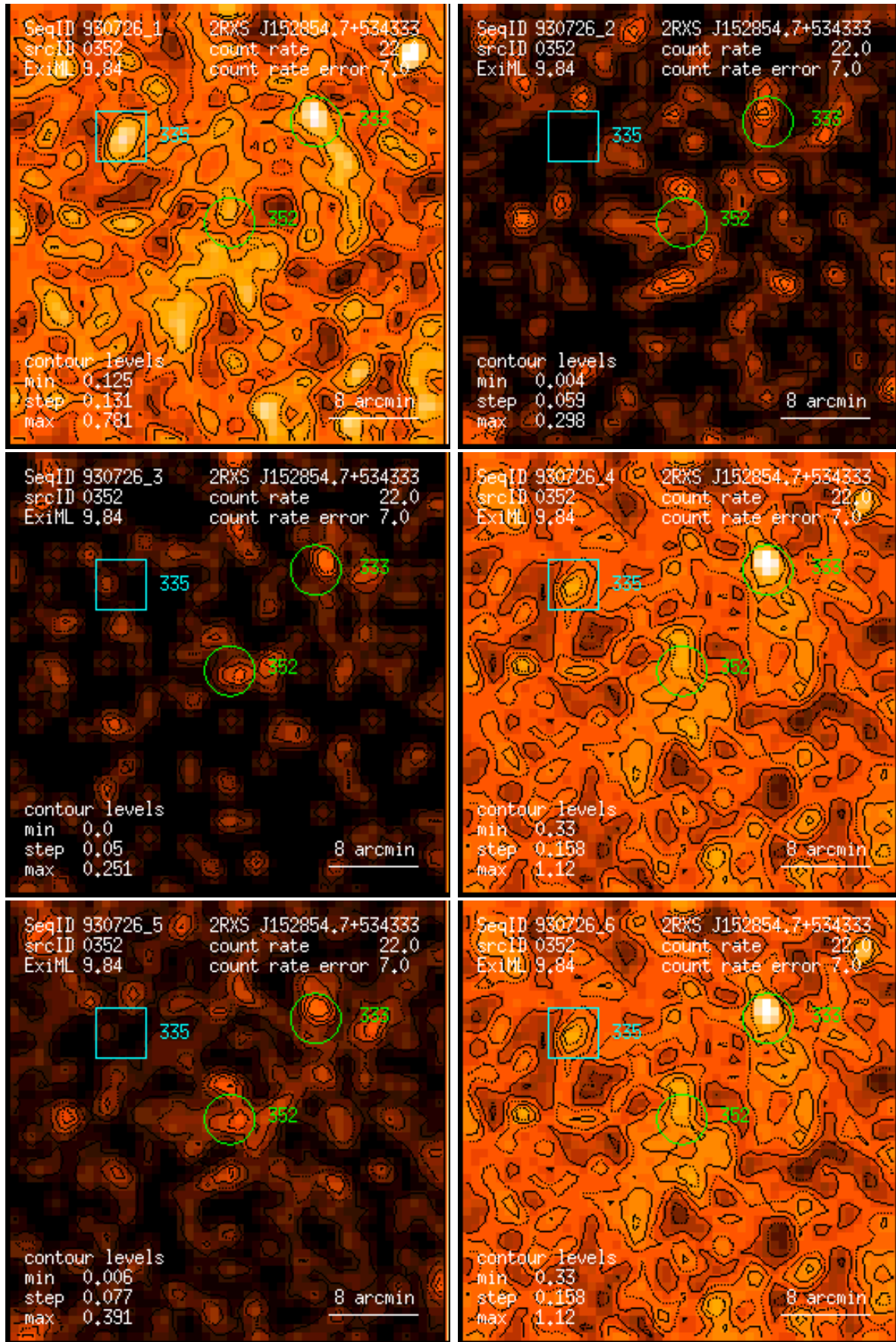
Figure 352: RASS 930726: detection 0352: band rate images, Gaussian filter: (1) PSPC channels 11 – 41, (2) 52 – 90, (3) 91 – 201, (4) 11 – 235, (5) 52 – 201, (6) 11 – 201. Broad band rates in counts/ks. Band rate contour levels in counts/ks/arcmin 2 .
