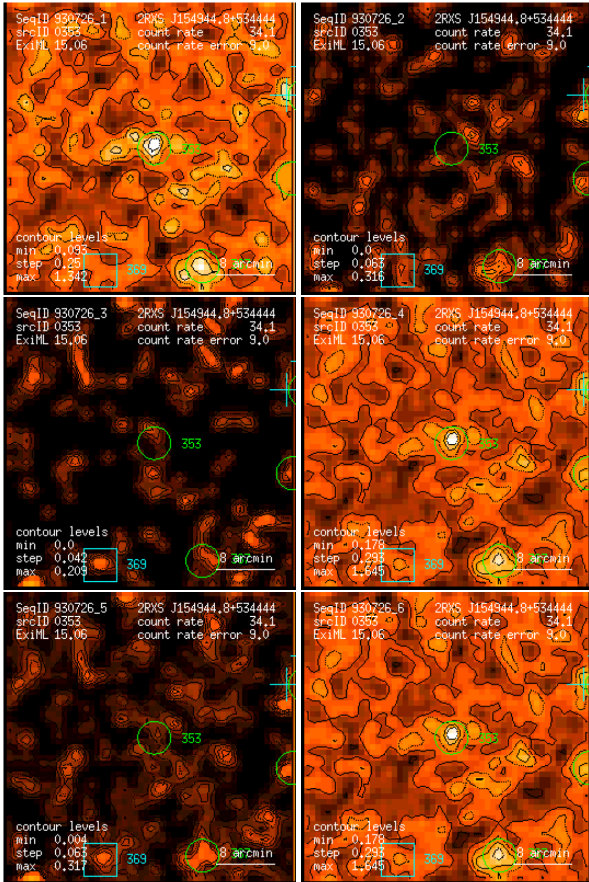
Figure 353: RASS 930726: detection 0353: band rate images, Gaussian filter: (1) PSPC channels 11 – 41, (2) 52 – 90, (3) 91 – 201, (4) 11 – 235, (5) 52 – 201, (6) 11 – 201. Broad band rates in counts/ks. Band rate contour levels in counts/ks/arcmin 2 .
