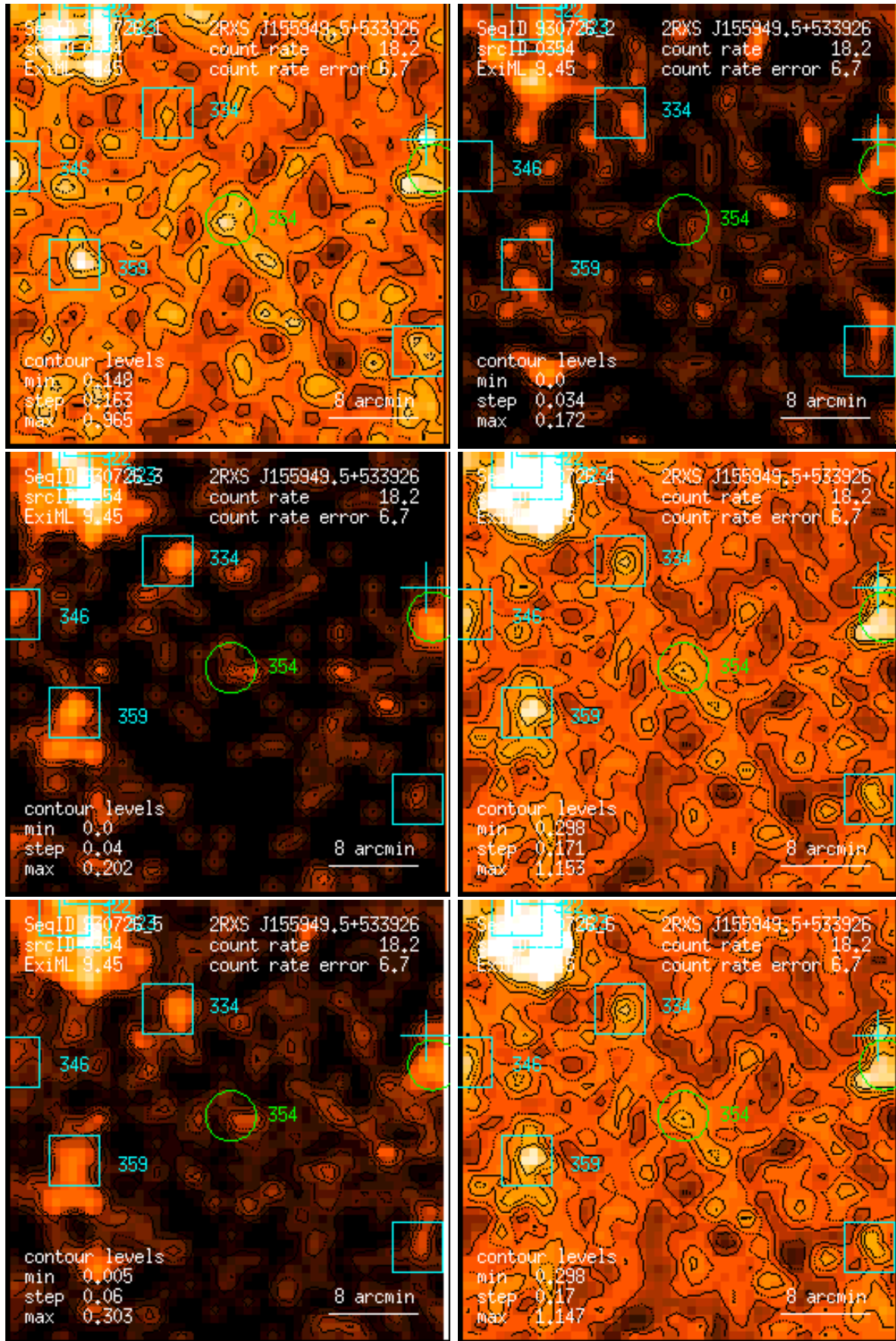
Figure 354: RASS 930726: detection 0354: band rate images, Gaussian filter: (1) PSPC channels 11 – 41, (2) 52 – 90, (3) 91 – 201, (4) 11 – 235, (5) 52 – 201, (6) 11 – 201. Broad band rates in counts/ks. Band rate contour levels in counts/ks/arcmin 2 .
