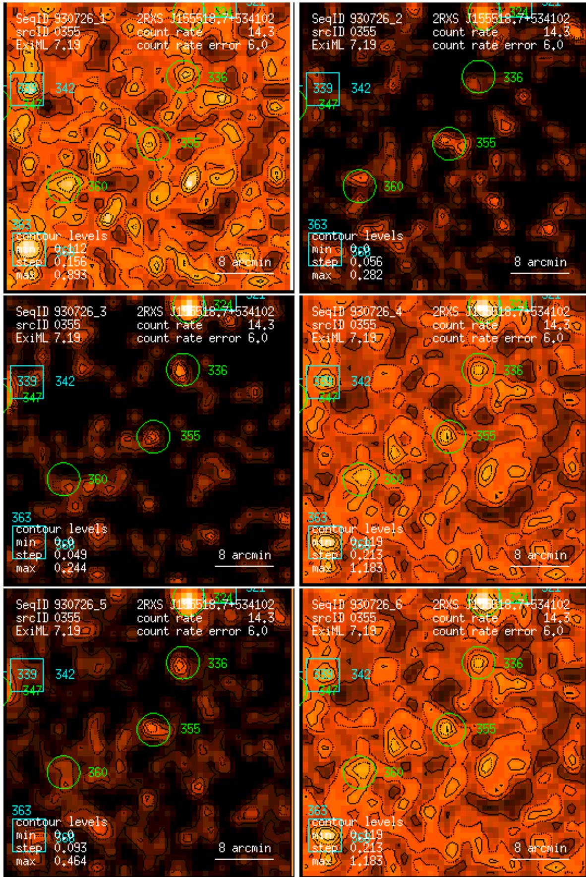
Figure 355: RASS 930726: detection 0355: band rate images, Gaussian filter: (1) PSPC channels 11 – 41, (2) 52 – 90, (3) 91 – 201, (4) 11 – 235, (5) 52 – 201, (6) 11 – 201. Broad band rates in counts/ks. Band rate contour levels in counts/ks/arcmin 2 .
