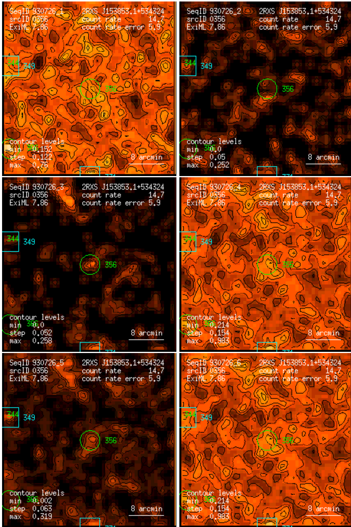
Figure 356: RASS 930726: detection 0356: band rate images, Gaussian filter: (1) PSPC channels 11 – 41, (2) 52 – 90, (3) 91 – 201, (4) 11 – 235, (5) 52 – 201, (6) 11 – 201. Broad band rates in counts/ks. Band rate contour levels in counts/ks/arcmin 2 .
