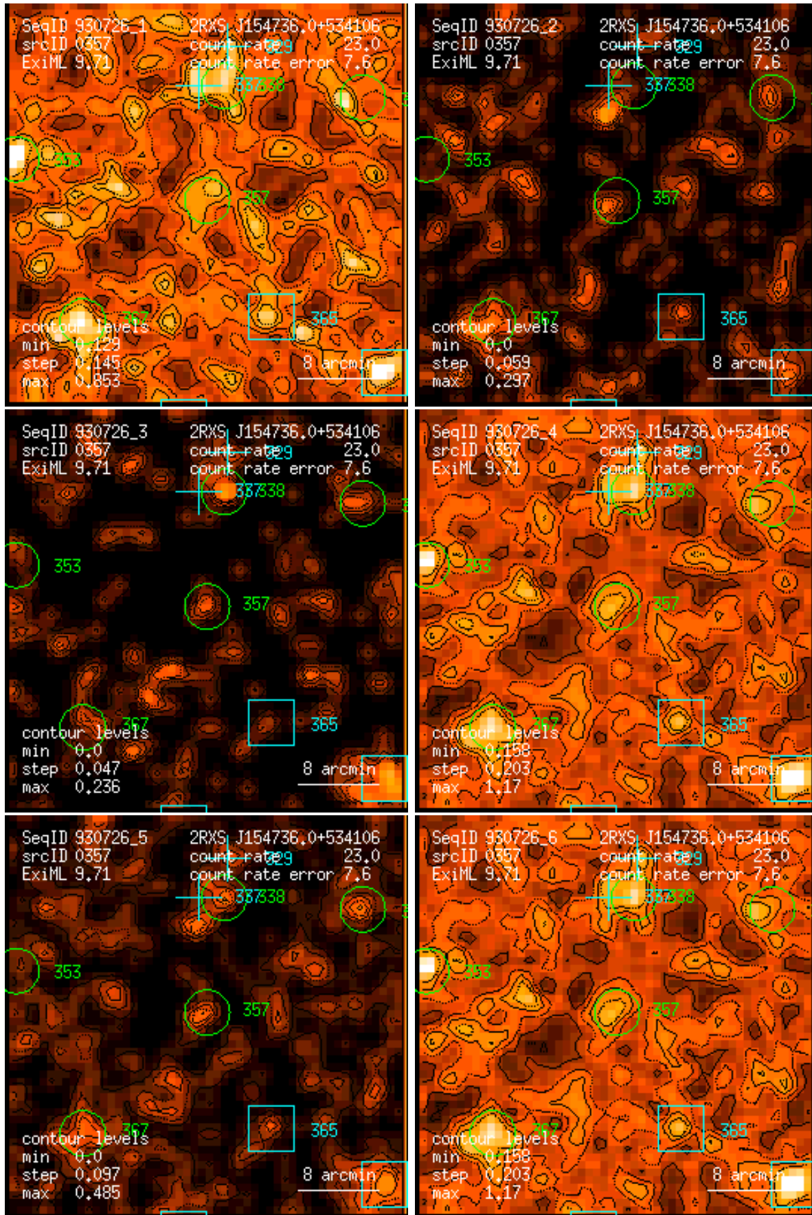
Figure 357: RASS 930726: detection 0357: band rate images, Gaussian filter: (1) PSPC channels 11 – 41, (2) 52 – 90, (3) 91 – 201, (4) 11 – 235, (5) 52 – 201, (6) 11 – 201. Broad band rates in counts/ks. Band rate contour levels in counts/ks/arcmin 2 .
