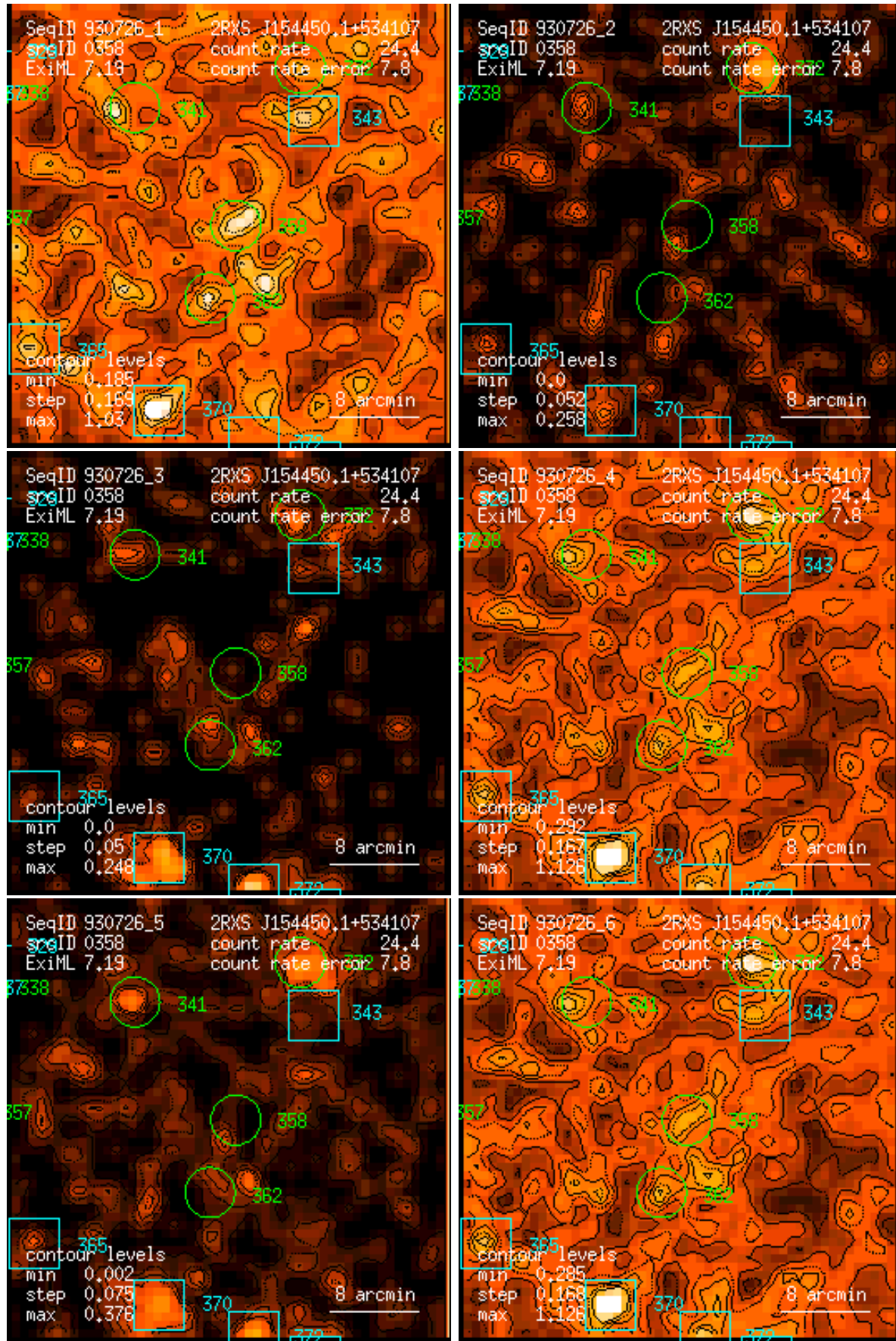
Figure 358: RASS 930726: detection 0358: band rate images, Gaussian filter: (1) PSPC channels 11 – 41, (2) 52 – 90, (3) 91 – 201, (4) 11 – 235, (5) 52 – 201, (6) 11 – 201. Broad band rates in counts/ks. Band rate contour levels in counts/ks/arcmin 2 .
