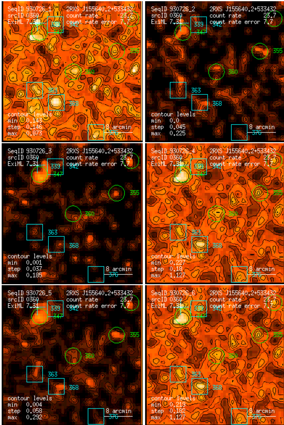
Figure 360: RASS 930726: detection 0360: band rate images, Gaussian filter: (1) PSPC channels 11 – 41, (2) 52 – 90, (3) 91 – 201, (4) 11 – 235, (5) 52 – 201, (6) 11 – 201. Broad band rates in counts/ks. Band rate contour levels in counts/ks/arcmin 2 .
