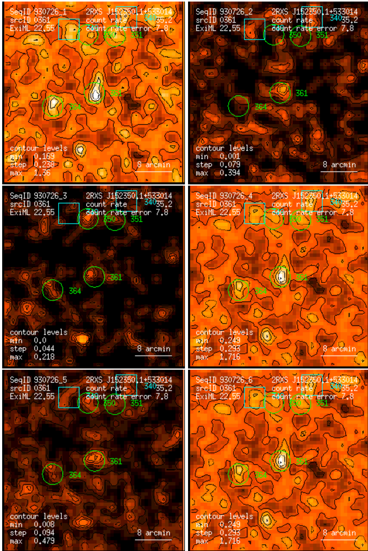
Figure 361: RASS 930726: detection 0361: band rate images, Gaussian filter: (1) PSPC channels 11 – 41, (2) 52 – 90, (3) 91 – 201, (4) 11 – 235, (5) 52 – 201, (6) 11 – 201. Broad band rates in counts/ks. Band rate contour levels in counts/ks/arcmin 2 .
