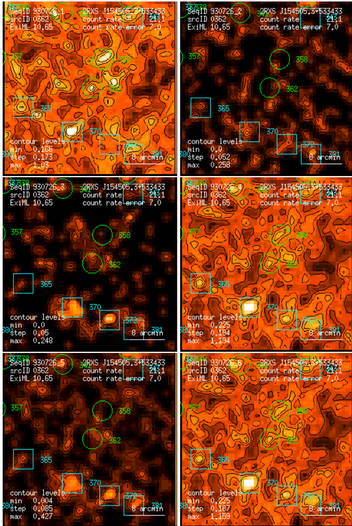
Figure 362: RASS 930726: detection 0362: band rate images, Gaussian filter: (1) PSPC channels 11 – 41, (2) 52 – 90, (3) 91 – 201, (4) 11 – 235, (5) 52 – 201, (6) 11 – 201. Broad band rates in counts/ks. Band rate contour levels in counts/ks/arcmin 2 .
