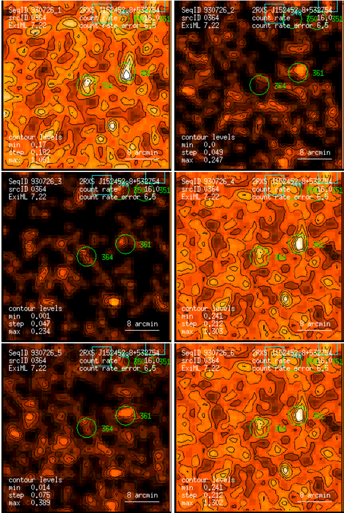
Figure 364: RASS 930726: detection 0364: band rate images, Gaussian filter: (1) PSPC channels 11 – 41, (2) 52 – 90, (3) 91 – 201, (4) 11 – 235, (5) 52 – 201, (6) 11 – 201. Broad band rates in counts/ks. Band rate contour levels in counts/ks/arcmin 2 .
