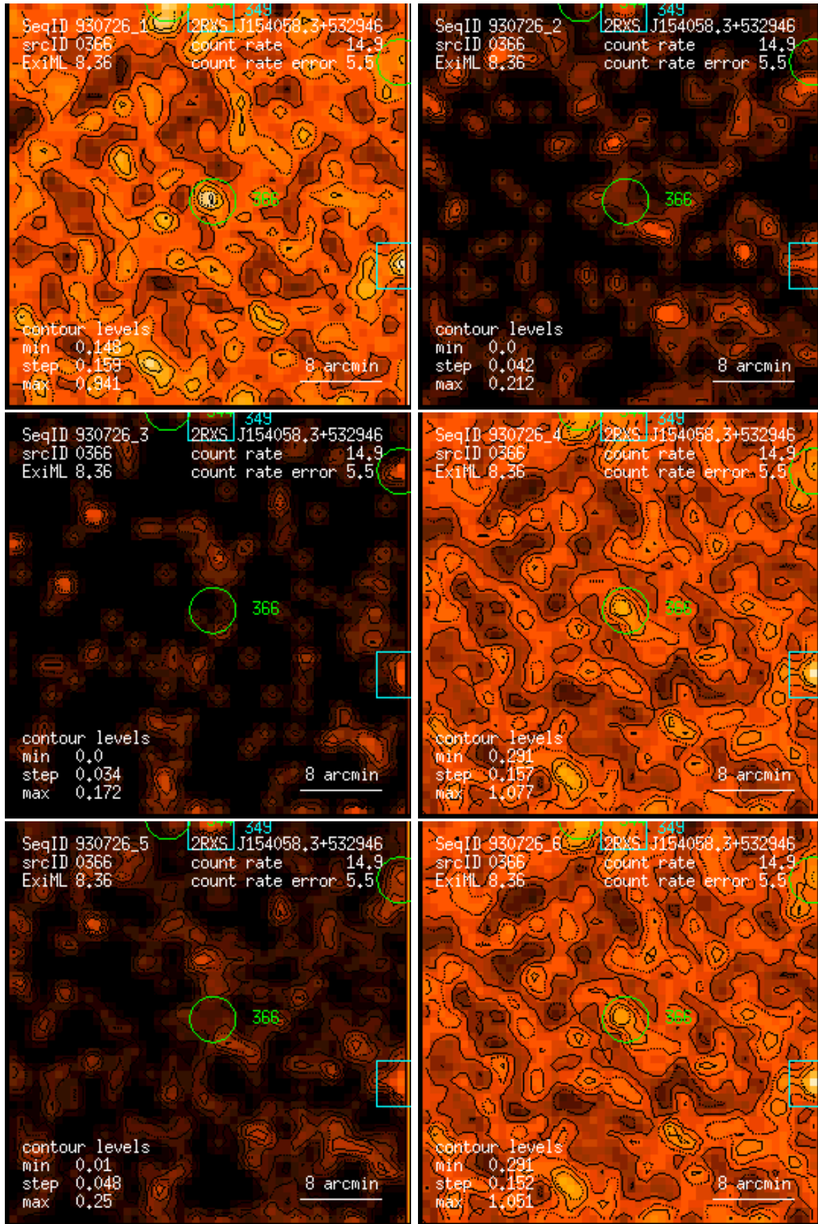
Figure 366: RASS 930726: detection 0366: band rate images, Gaussian filter: (1) PSPC channels 11 – 41, (2) 52 – 90, (3) 91 – 201, (4) 11 – 235, (5) 52 – 201, (6) 11 – 201. Broad band rates in counts/ks. Band rate contour levels in counts/ks/arcmin 2 .
