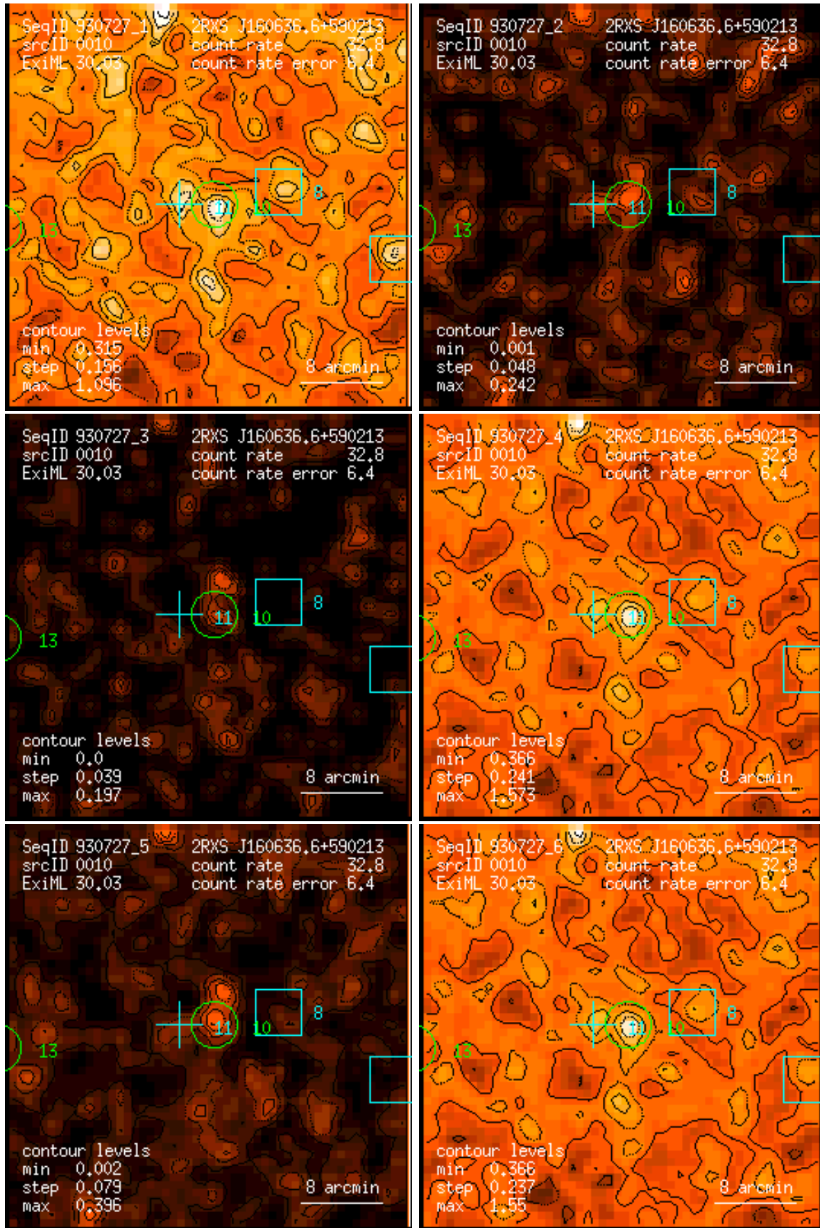
Figure 10: RASS 930727: detection 0010: band rate images, Gaussian filter: (1) PSPC channels 11 – 41, (2) 52 – 90, (3) 91 – 201, (4) 11 – 235, (5) 52 – 201, (6) 11 – 201. Broad band rates in counts/ks. Band rate contour levels in counts/ks/arcmin 2 .
