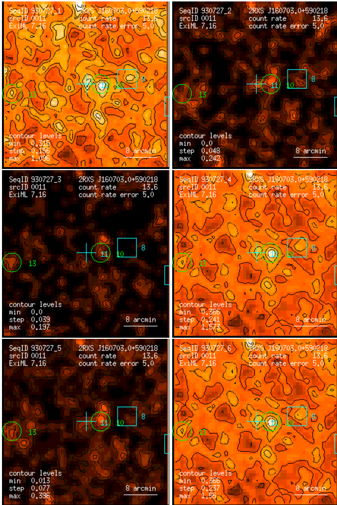
Figure 11: RASS 930727: detection 0011: band rate images, Gaussian filter: (1) PSPC channels 11 – 41, (2) 52 – 90, (3) 91 – 201, (4) 11 – 235, (5) 52 – 201, (6) 11 – 201. Broad band rates in counts/ks. Band rate contour levels in counts/ks/arcmin 2 .
