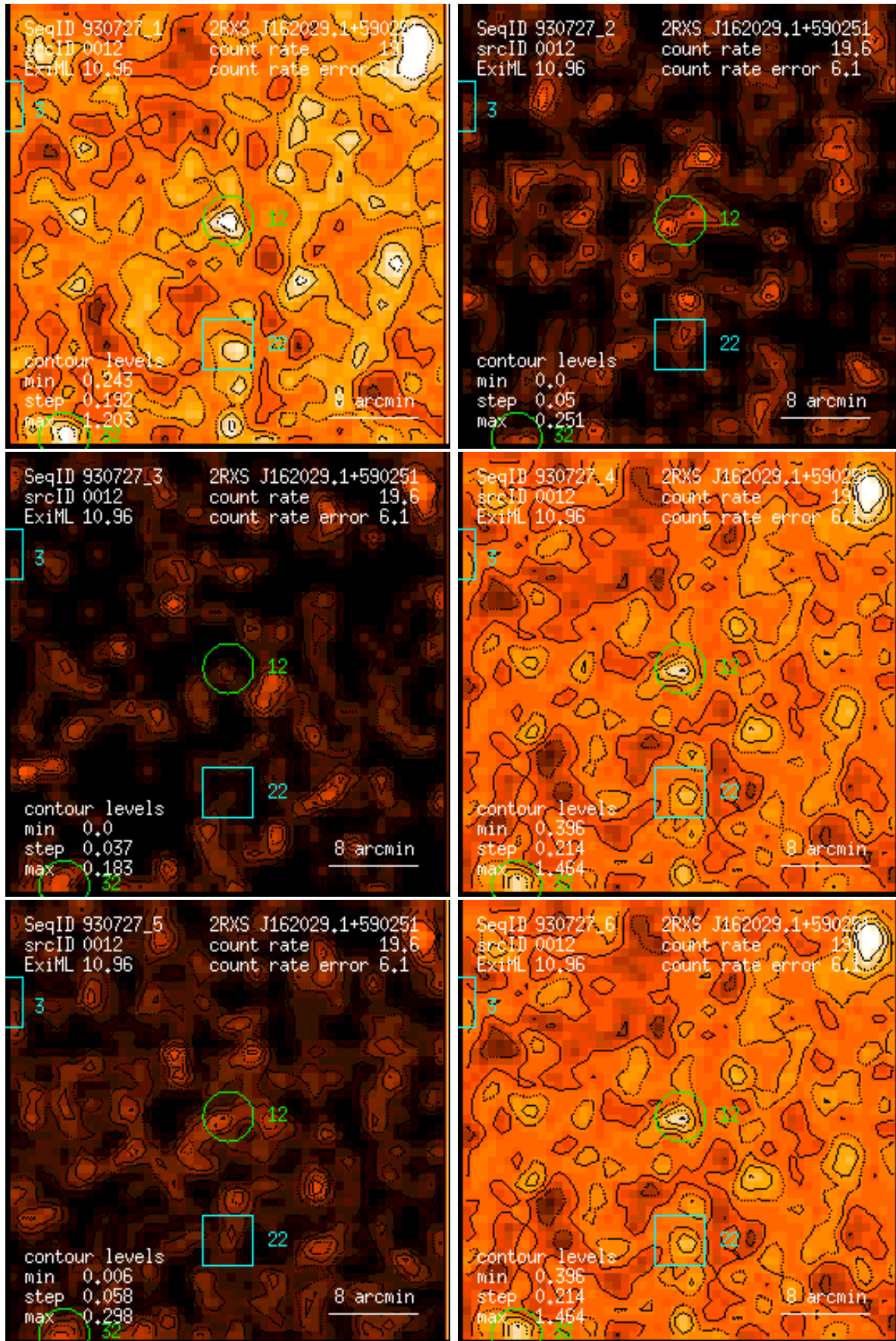
Figure 12: RASS 930727: detection 0012: band rate images, Gaussian filter: (1) PSPC channels 11 – 41, (2) 52 – 90, (3) 91 – 201, (4) 11 – 235, (5) 52 – 201, (6) 11 – 201. Broad band rates in counts/ks. Band rate contour levels in counts/ks/arcmin 2 .
