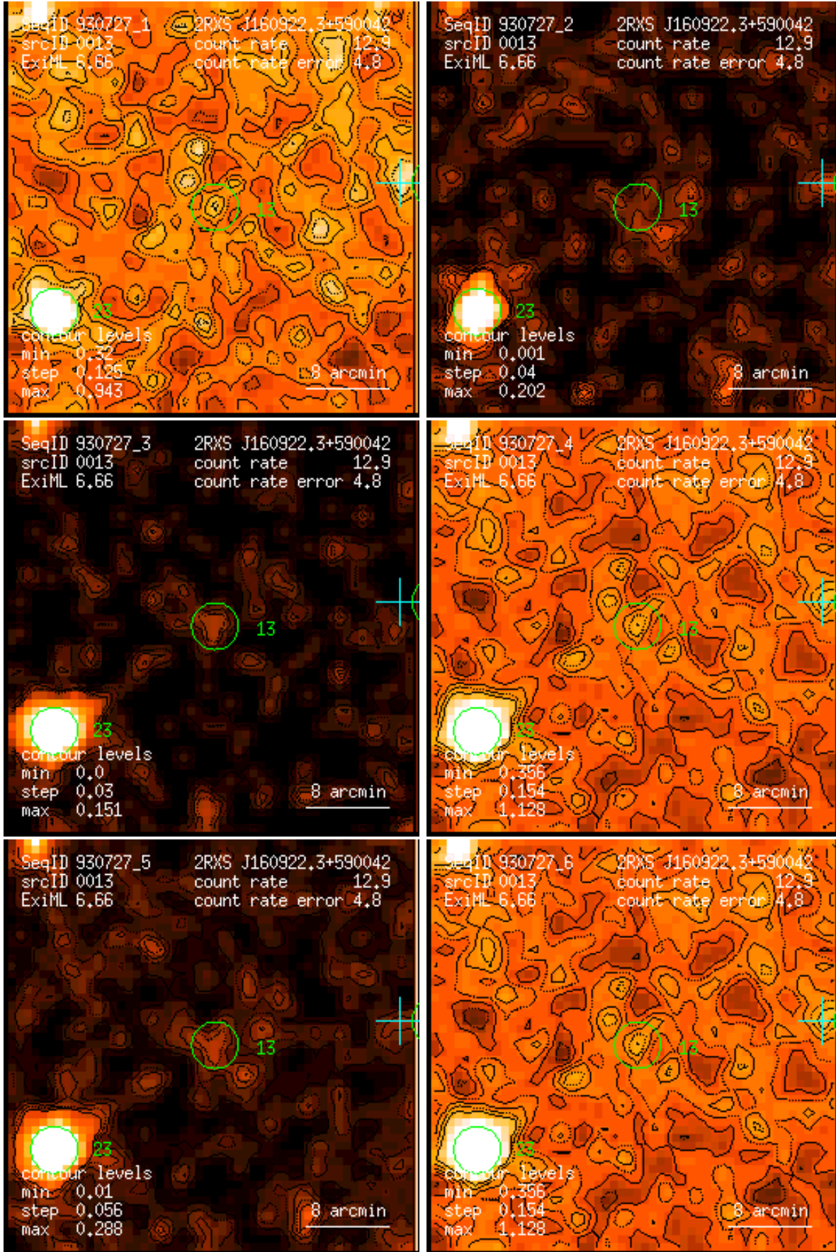
Figure 13: RASS 930727: detection 0013: band rate images, Gaussian filter: (1) PSPC channels 11 – 41, (2) 52 – 90, (3) 91 – 201, (4) 11 – 235, (5) 52 – 201, (6) 11 – 201. Broad band rates in counts/ks. Band rate contour levels in counts/ks/arcmin 2 .
