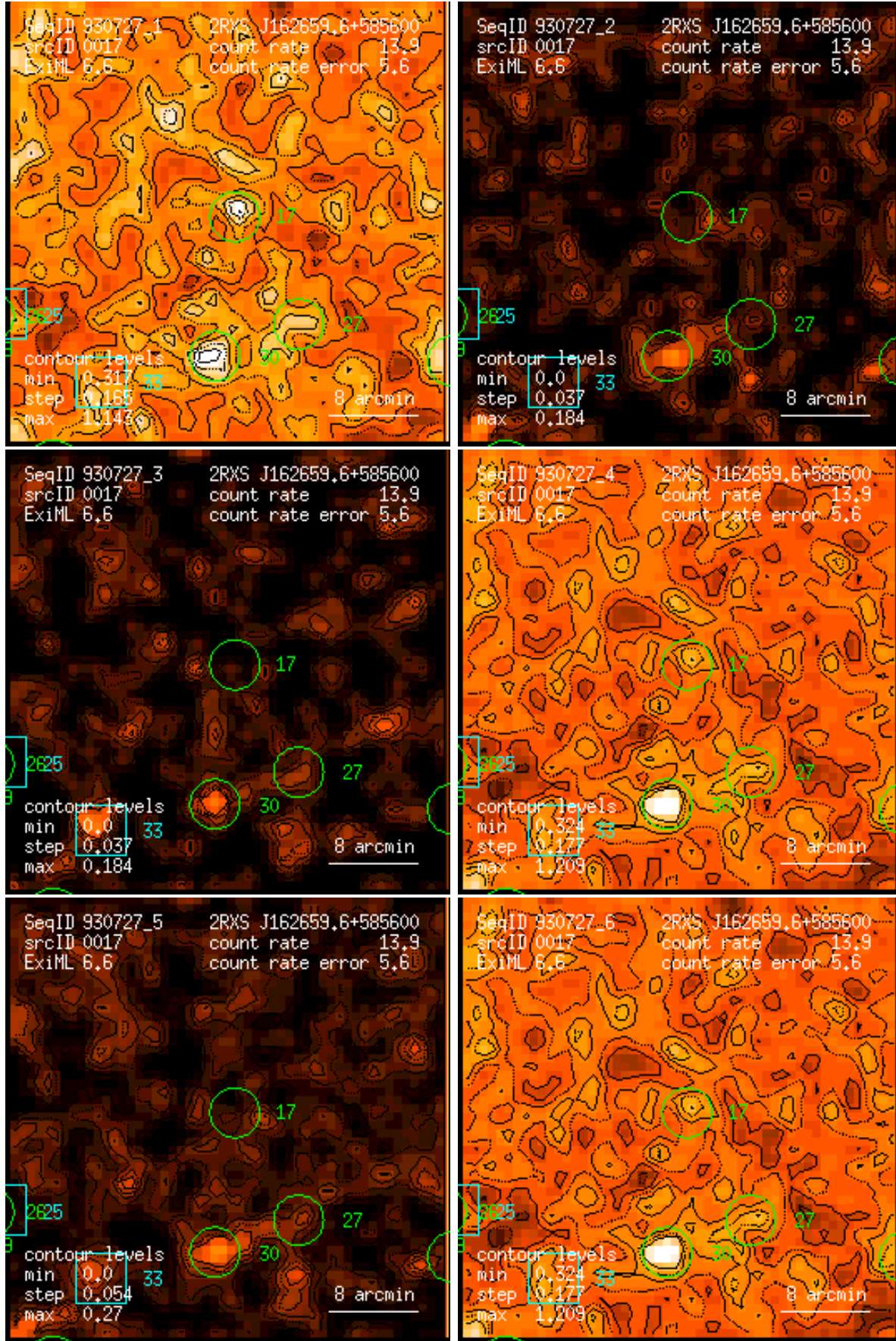
Figure 17: RASS 930727: detection 0017: band rate images, Gaussian filter: (1) PSPC channels 11 – 41, (2) 52 – 90, (3) 91 – 201, (4) 11 – 235, (5) 52 – 201, (6) 11 – 201. Broad band rates in counts/ks. Band rate contour levels in counts/ks/arcmin 2 .
