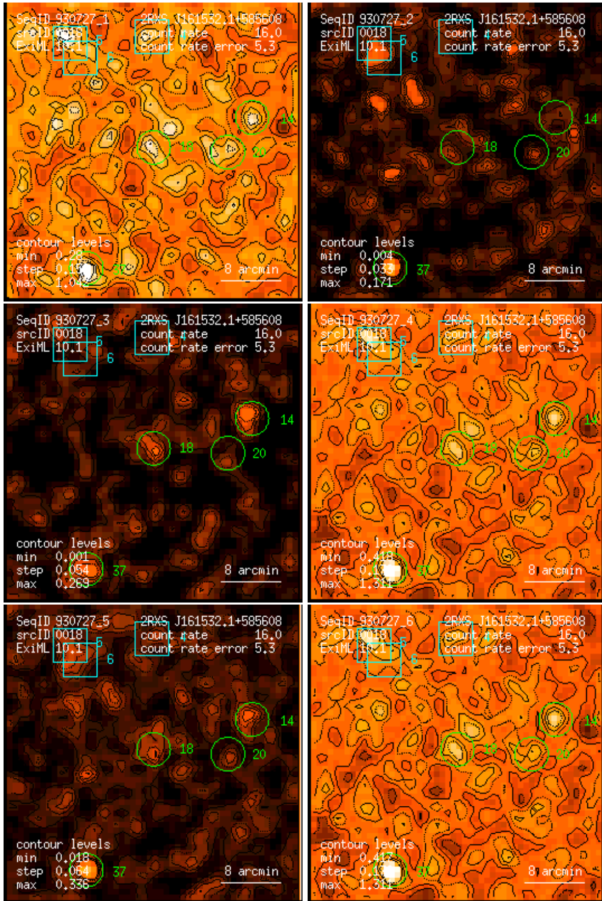
Figure 18: RASS 930727: detection 0018: band rate images, Gaussian filter: (1) PSPC channels 11 – 41, (2) 52 – 90, (3) 91 – 201, (4) 11 – 235, (5) 52 – 201, (6) 11 – 201. Broad band rates in counts/ks. Band rate contour levels in counts/ks/arcmin 2 .
