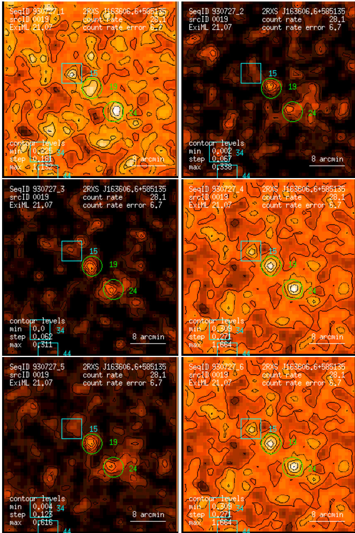
Figure 19: RASS 930727: detection 0019: band rate images, Gaussian filter: (1) PSPC channels 11 – 41, (2) 52 – 90, (3) 91 – 201, (4) 11 – 235, (5) 52 – 201, (6) 11 – 201. Broad band rates in counts/ks. Band rate contour levels in counts/ks/arcmin 2 .
